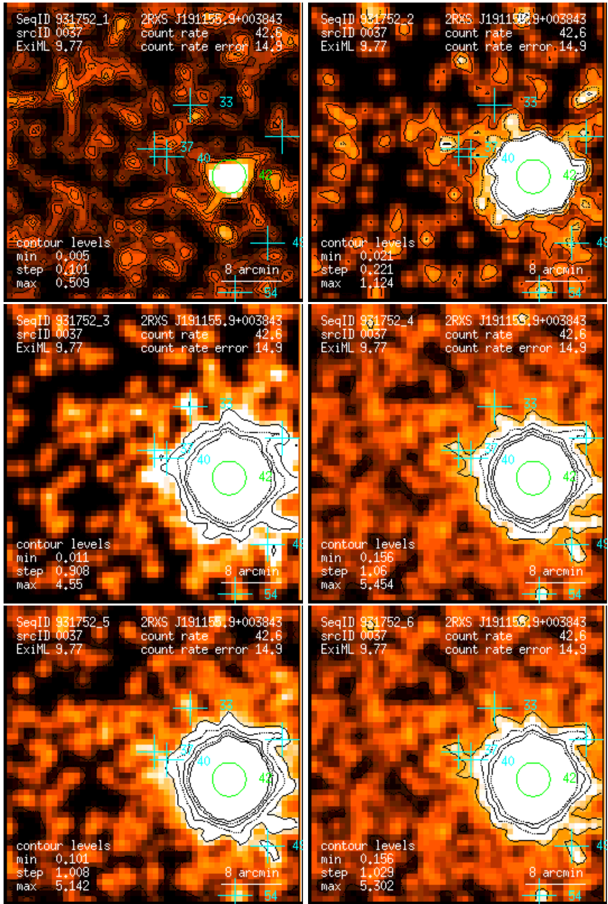
Figure 37: RASS 931752: detection 0037: band rate images, Gaussian filter: (1) PSPC channels 11 – 41, (2) 52 – 90, (3) 91 – 201, (4) 11 – 235, (5) 52 – 201, (6) 11 – 201. Broad band rates in counts/ks. Band rate contour levels in counts/ks/arcmin 2 .
