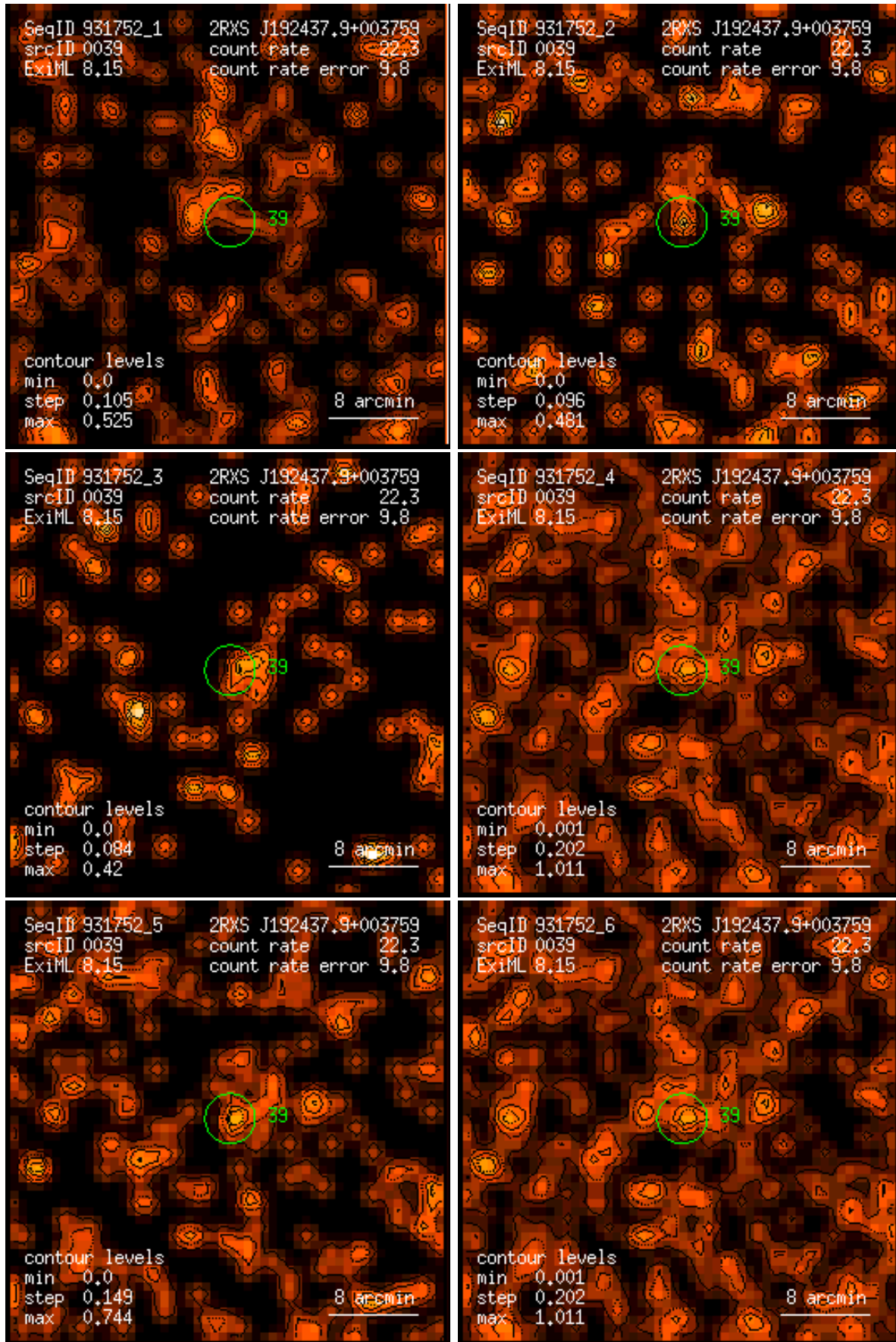
Figure 39: RASS 931752: detection 0039: band rate images, Gaussian filter: (1) PSPC channels 11 – 41, (2) 52 – 90, (3) 91 – 201, (4) 11 – 235, (5) 52 – 201, (6) 11 – 201. Broad band rates in counts/ks. Band rate contour levels in counts/ks/arcmin 2 .
