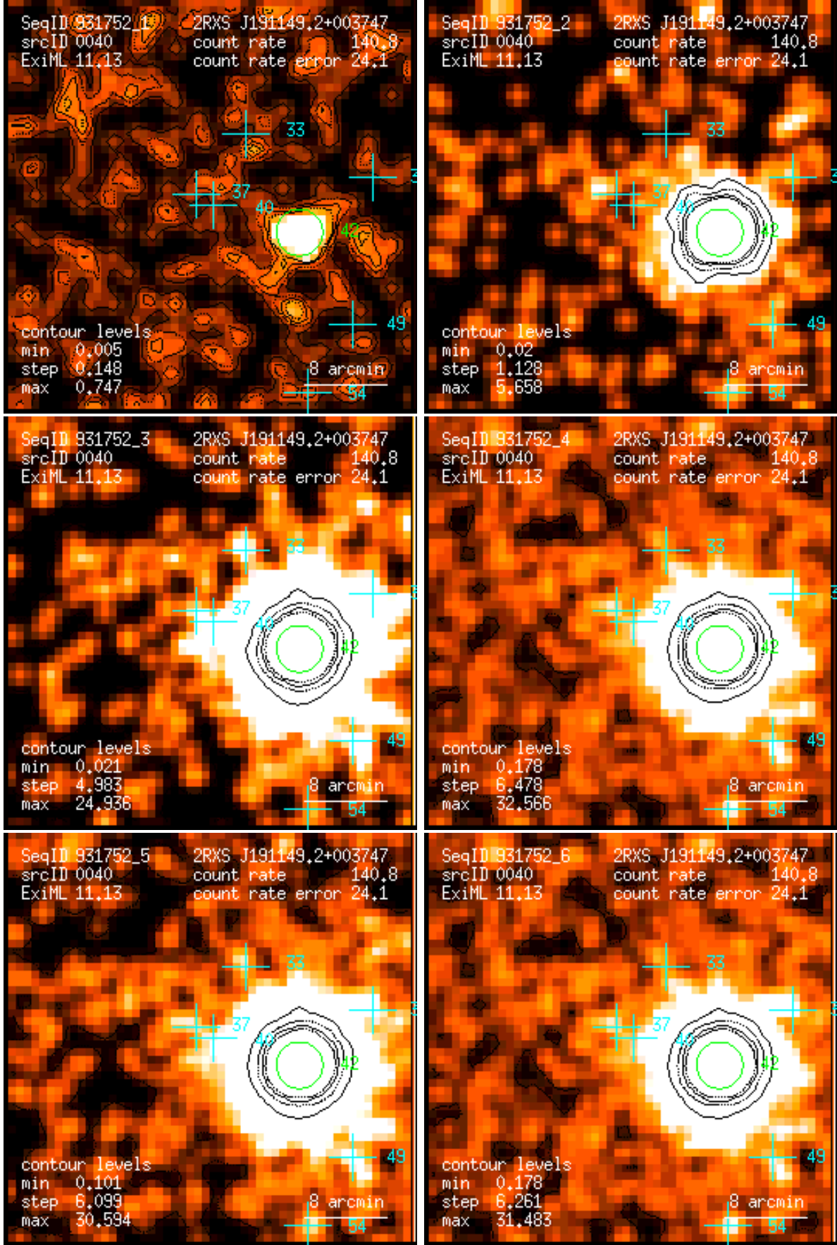
Figure 40: RASS 931752: detection 0040: band rate images, Gaussian filter: (1) PSPC channels 11 – 41, (2) 52 – 90, (3) 91 – 201, (4) 11 – 235, (5) 52 – 201, (6) 11 – 201. Broad band rates in counts/ks. Band rate contour levels in counts/ks/arcmin 2 .
