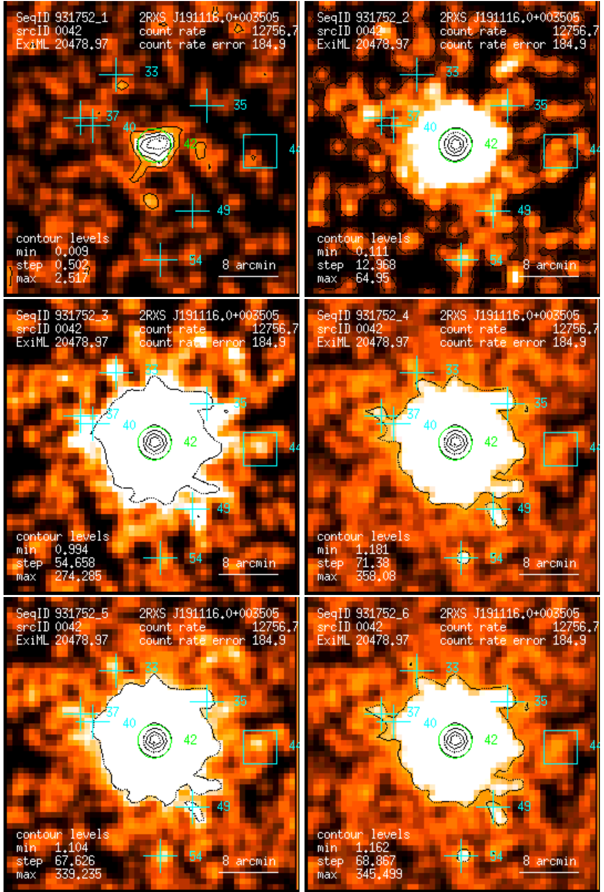
Figure 42: RASS 931752: detection 0042: band rate images, Gaussian filter: (1) PSPC channels 11 – 41, (2) 52 – 90, (3) 91 – 201, (4) 11 – 235, (5) 52 – 201, (6) 11 – 201. Broad band rates in counts/ks. Band rate contour levels in counts/ks/arcmin 2 .
