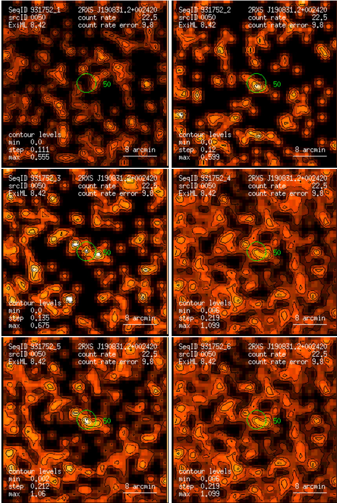
Figure 50: RASS 931752: detection 0050: band rate images, Gaussian filter: (1) PSPC channels 11 – 41, (2) 52 – 90, (3) 91 – 201, (4) 11 – 235, (5) 52 – 201, (6) 11 – 201. Broad band rates in counts/ks. Band rate contour levels in counts/ks/arcmin 2 .
