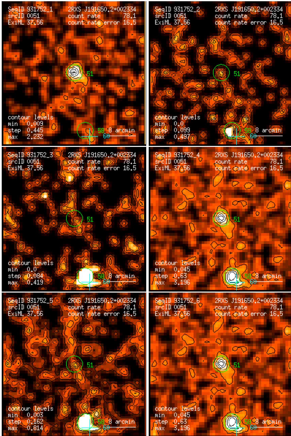
Figure 51: RASS 931752: detection 0051: band rate images, Gaussian filter: (1) PSPC channels 11 – 41, (2) 52 – 90, (3) 91 – 201, (4) 11 – 235, (5) 52 – 201, (6) 11 – 201. Broad band rates in counts/ks. Band rate contour levels in counts/ks/arcmin 2 .
