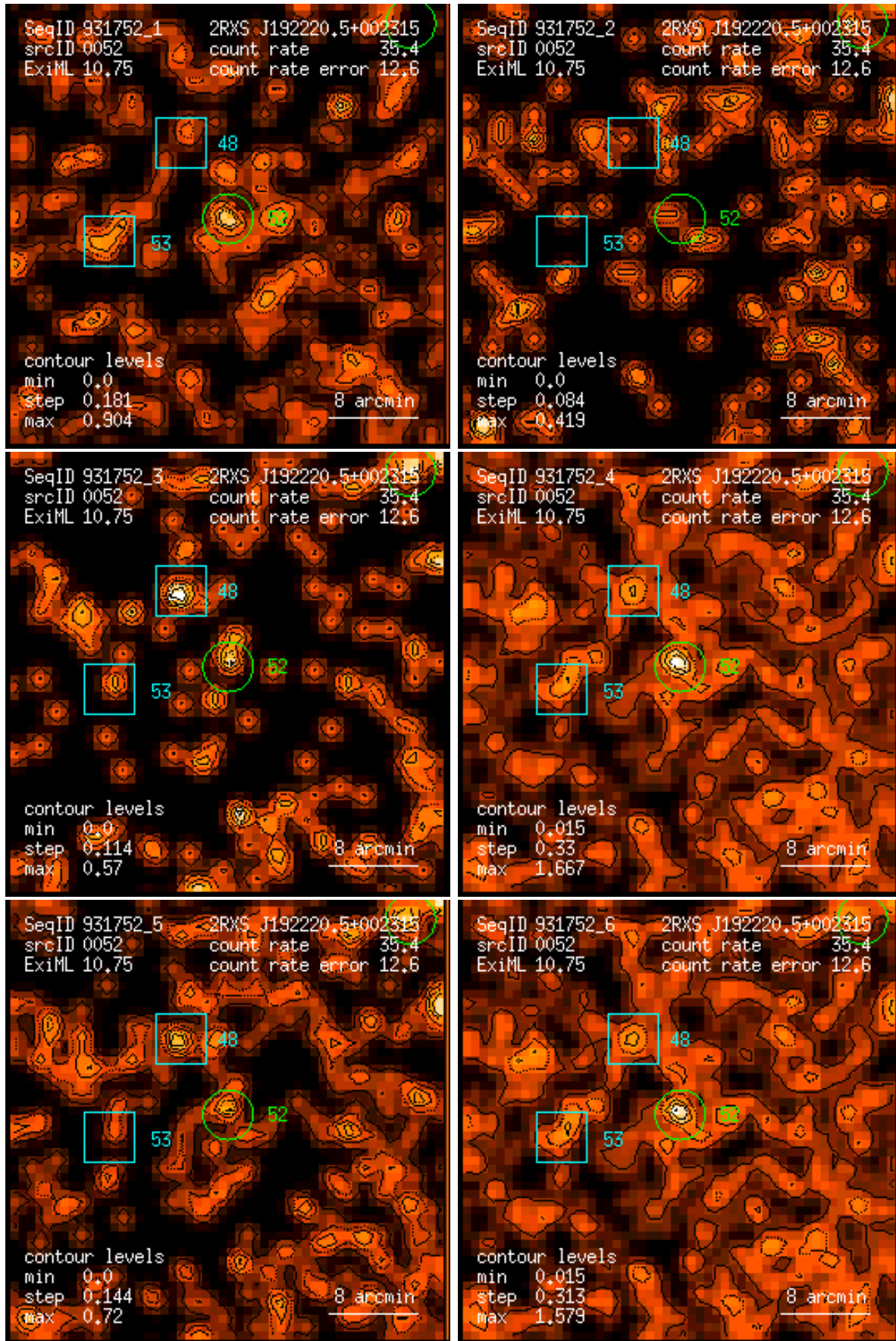
Figure 52: RASS 931752: detection 0052: band rate images, Gaussian filter: (1) PSPC channels 11 – 41, (2) 52 – 90, (3) 91 – 201, (4) 11 – 235, (5) 52 – 201, (6) 11 – 201. Broad band rates in counts/ks. Band rate contour levels in counts/ks/arcmin 2 .
