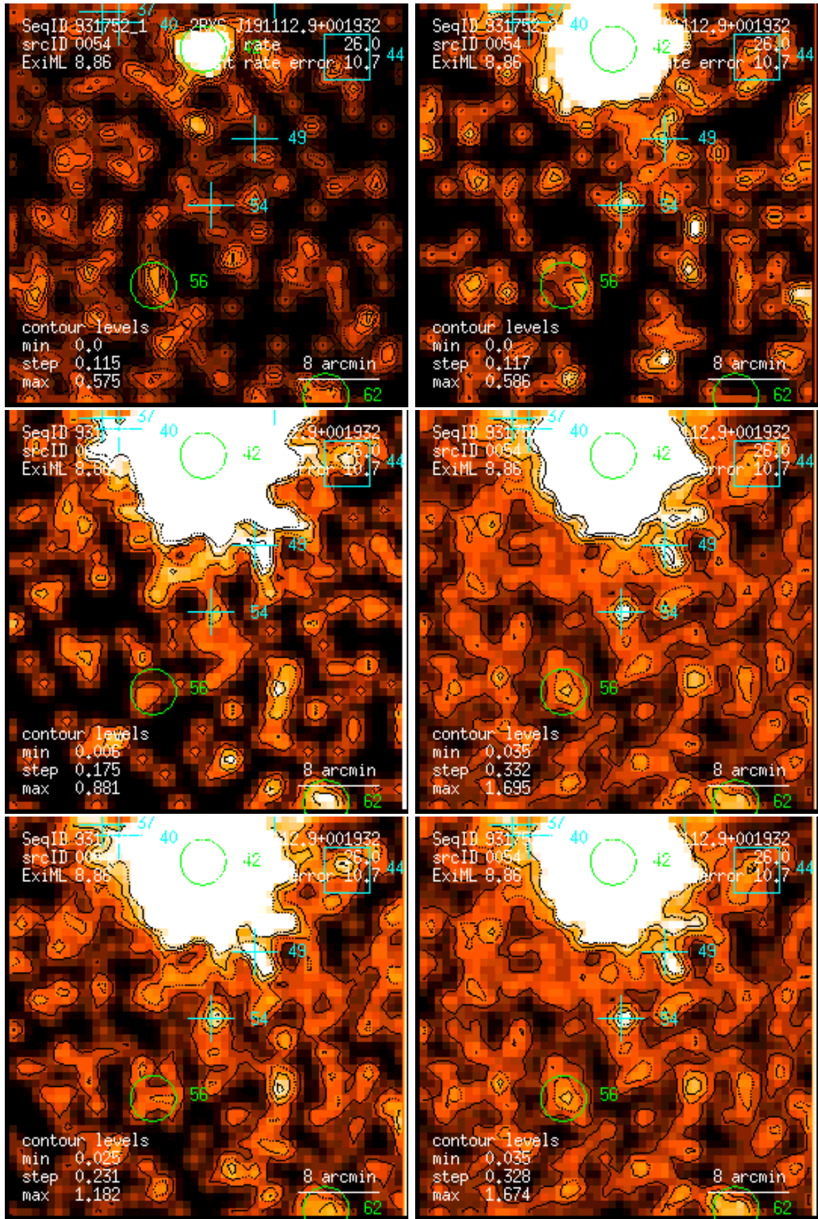
Figure 54: RASS 931752: detection 0054: band rate images, Gaussian filter: (1) PSPC channels 11 – 41, (2) 52 – 90, (3) 91 – 201, (4) 11 – 235, (5) 52 – 201, (6) 11 – 201. Broad band rates in counts/ks. Band rate contour levels in counts/ks/arcmin 2 .
