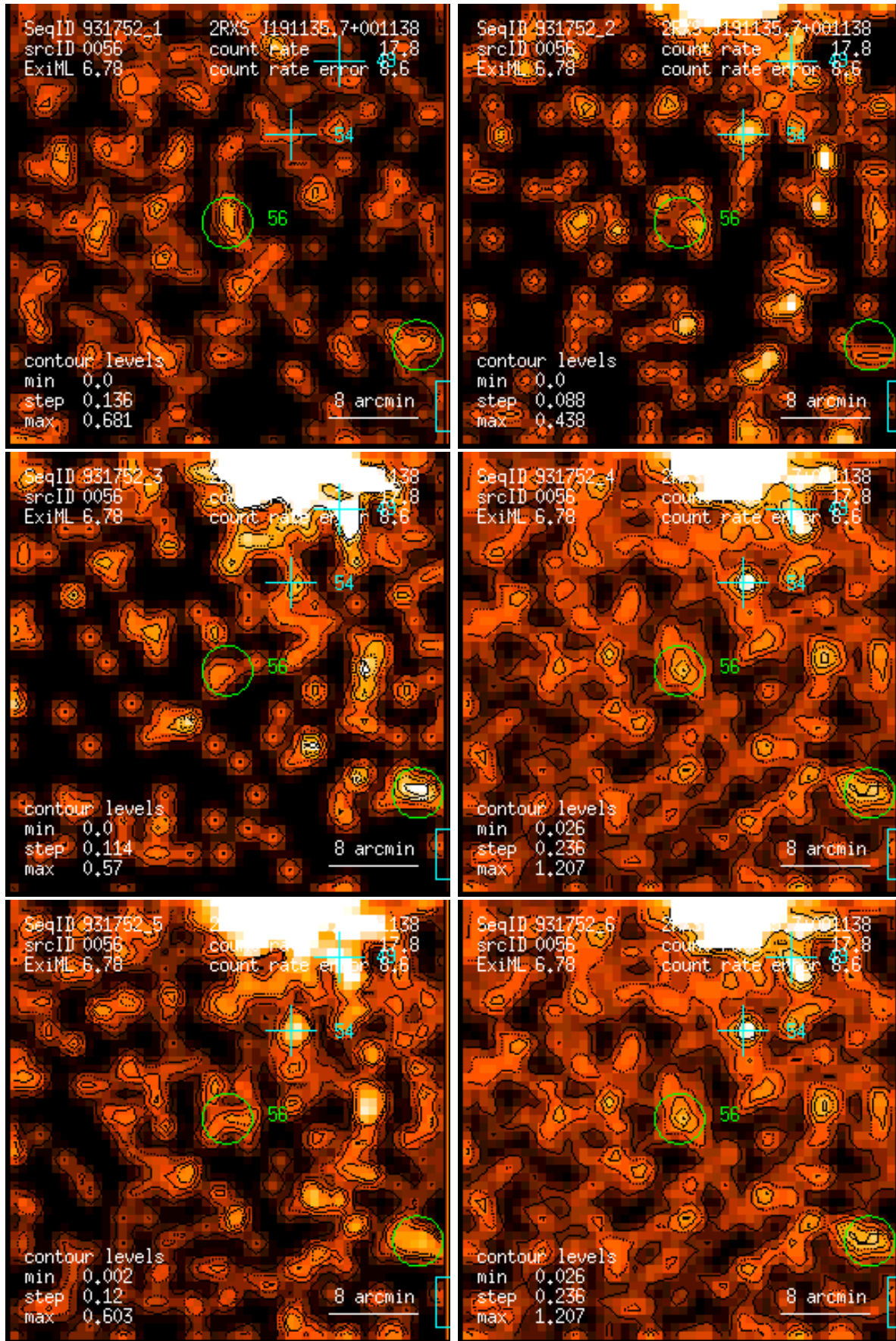
Figure 56: RASS 931752: detection 0056: band rate images, Gaussian filter: (1) PSPC channels 11 – 41, (2) 52 – 90, (3) 91 – 201, (4) 11 – 235, (5) 52 – 201, (6) 11 – 201. Broad band rates in counts/ks. Band rate contour levels in counts/ks/arcmin 2 .
