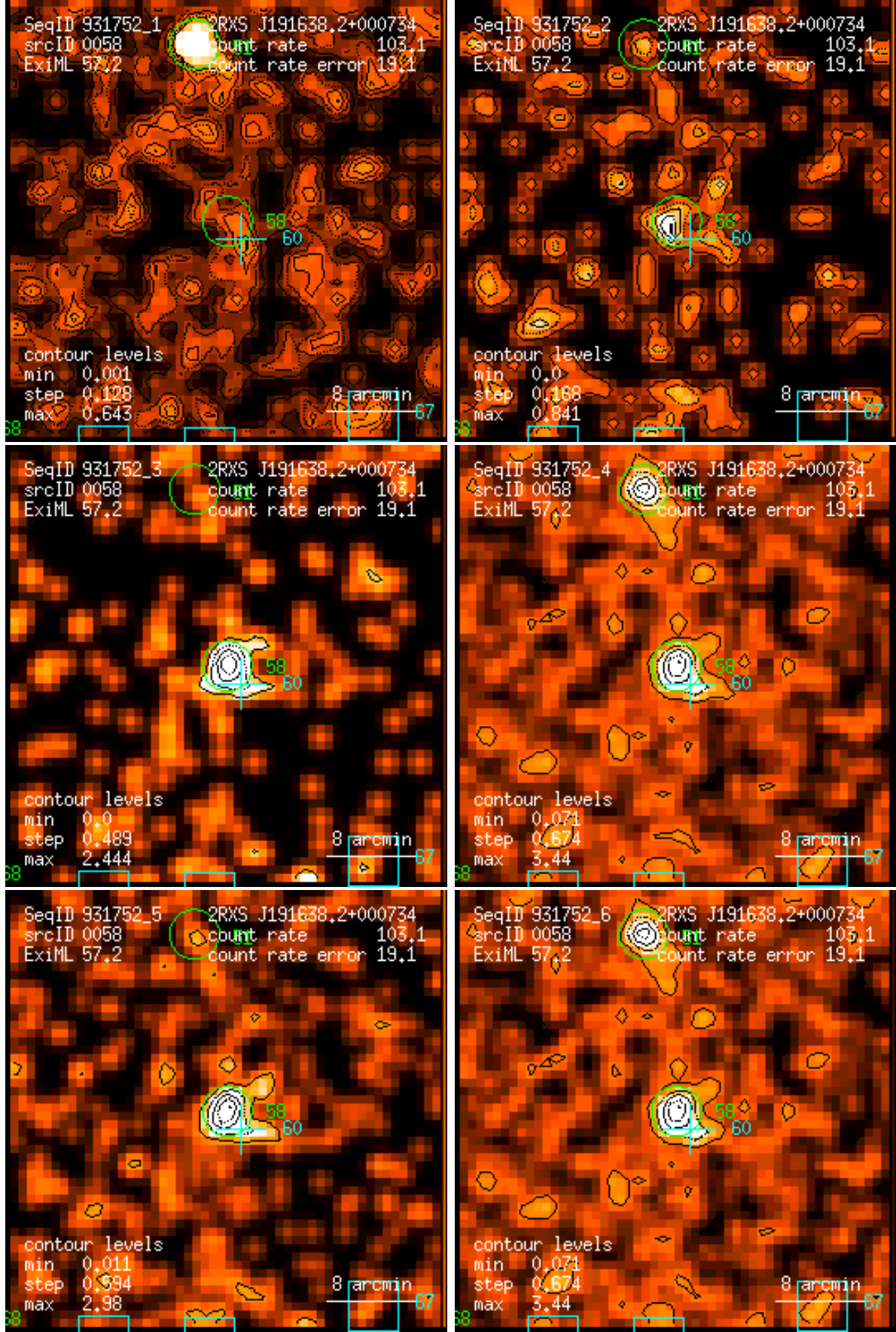
Figure 58: RASS 931752: detection 0058: band rate images, Gaussian filter: (1) PSPC channels 11 – 41, (2) 52 – 90, (3) 91 – 201, (4) 11 – 235, (5) 52 – 201, (6) 11 – 201. Broad band rates in counts/ks. Band rate contour levels in counts/ks/arcmin 2 .
