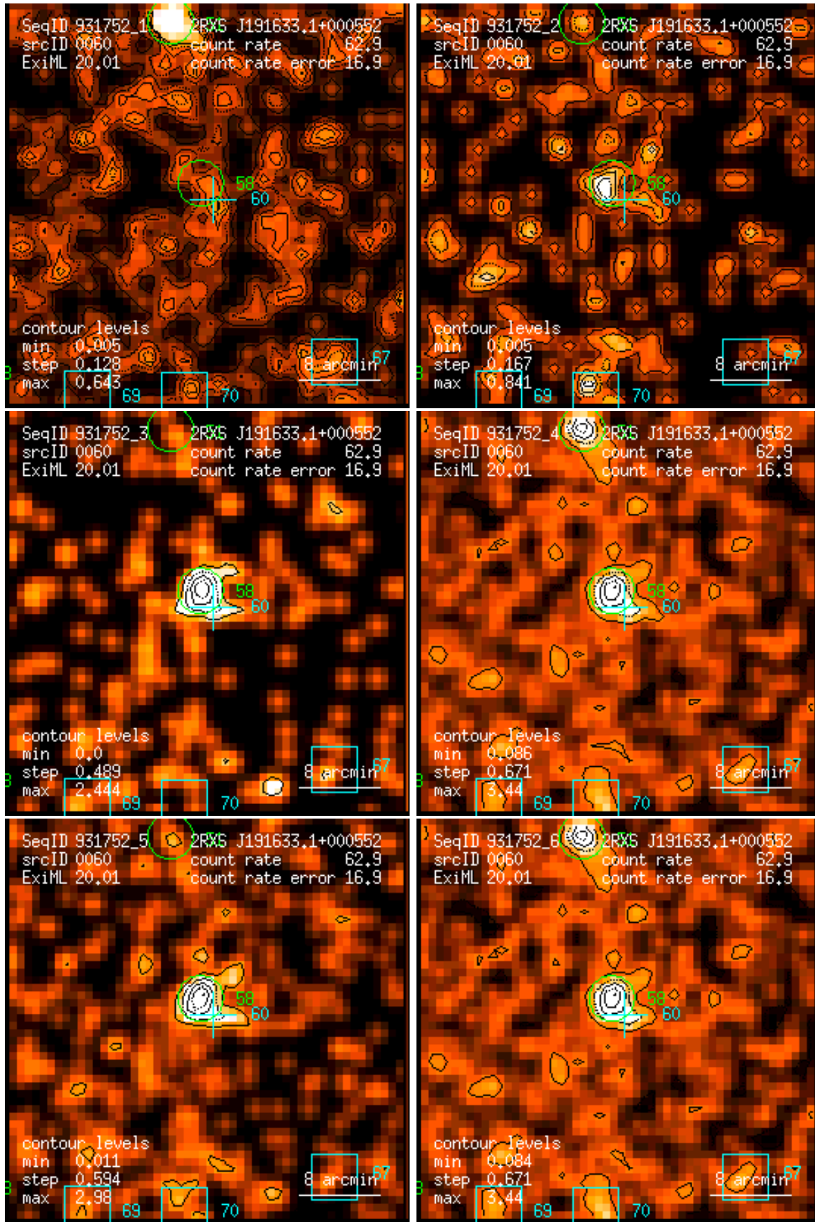
Figure 60: RASS 931752: detection 0060: band rate images, Gaussian filter: (1) PSPC channels 11 – 41, (2) 52 – 90, (3) 91 – 201, (4) 11 – 235, (5) 52 – 201, (6) 11 – 201. Broad band rates in counts/ks. Band rate contour levels in counts/ks/arcmin 2 .
