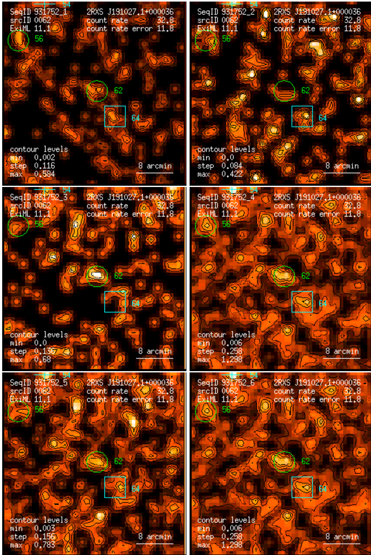
Figure 62: RASS 931752: detection 0062: band rate images, Gaussian filter: (1) PSPC channels 11 – 41, (2) 52 – 90, (3) 91 – 201, (4) 11 – 235, (5) 52 – 201, (6) 11 – 201. Broad band rates in counts/ks. Band rate contour levels in counts/ks/arcmin 2 .
