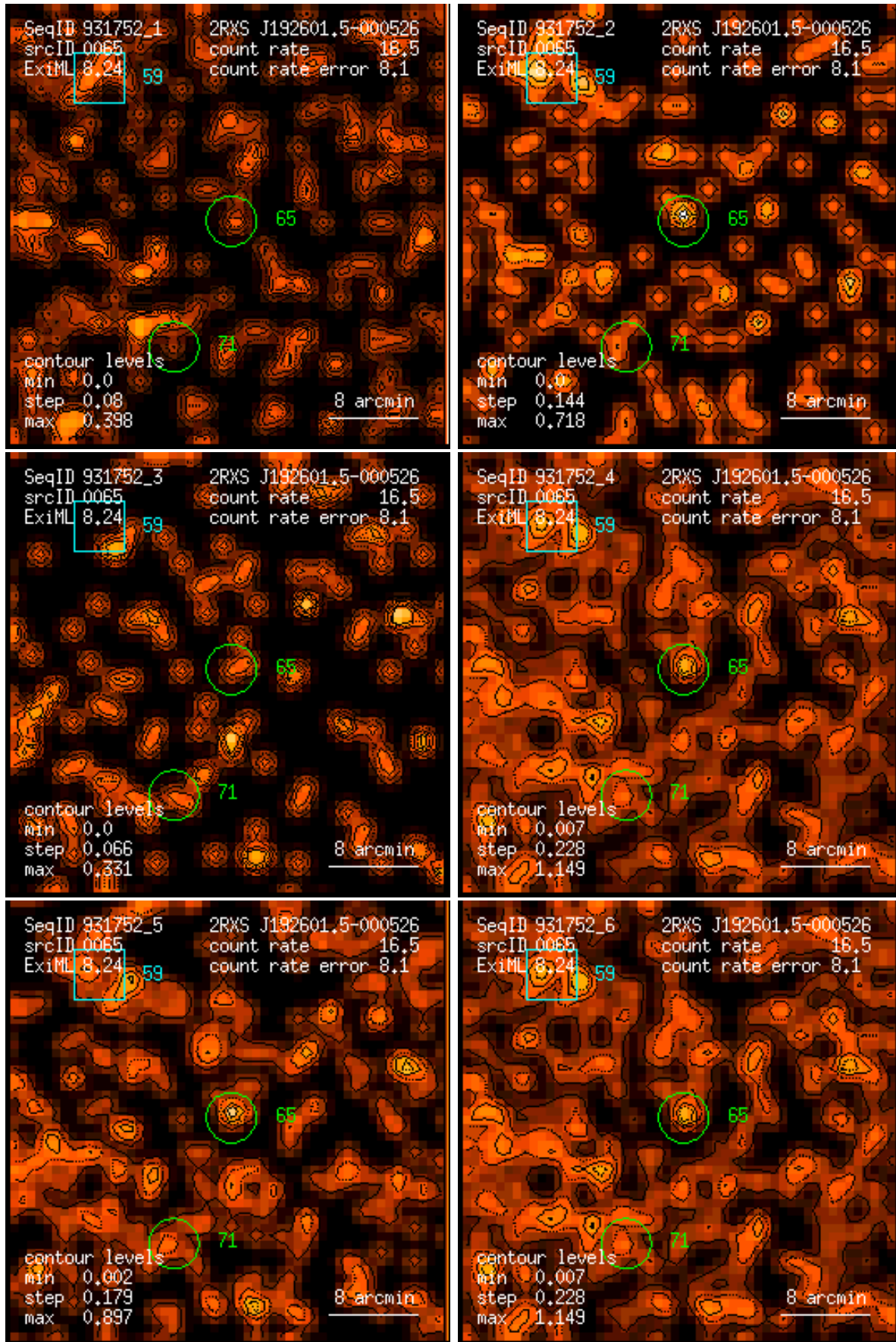
Figure 65: RASS 931752: detection 0065: band rate images, Gaussian filter: (1) PSPC channels 11 – 41, (2) 52 – 90, (3) 91 – 201, (4) 11 – 235, (5) 52 – 201, (6) 11 – 201. Broad band rates in counts/ks. Band rate contour levels in counts/ks/arcmin 2 .
