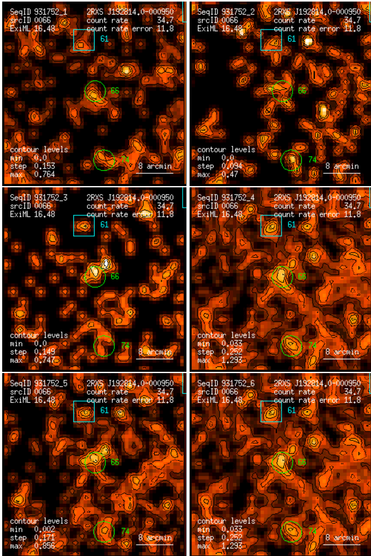
Figure 66: RASS 931752: detection 0066: band rate images, Gaussian filter: (1) PSPC channels 11 – 41, (2) 52 – 90, (3) 91 – 201, (4) 11 – 235, (5) 52 – 201, (6) 11 – 201. Broad band rates in counts/ks. Band rate contour levels in counts/ks/arcmin 2 .
