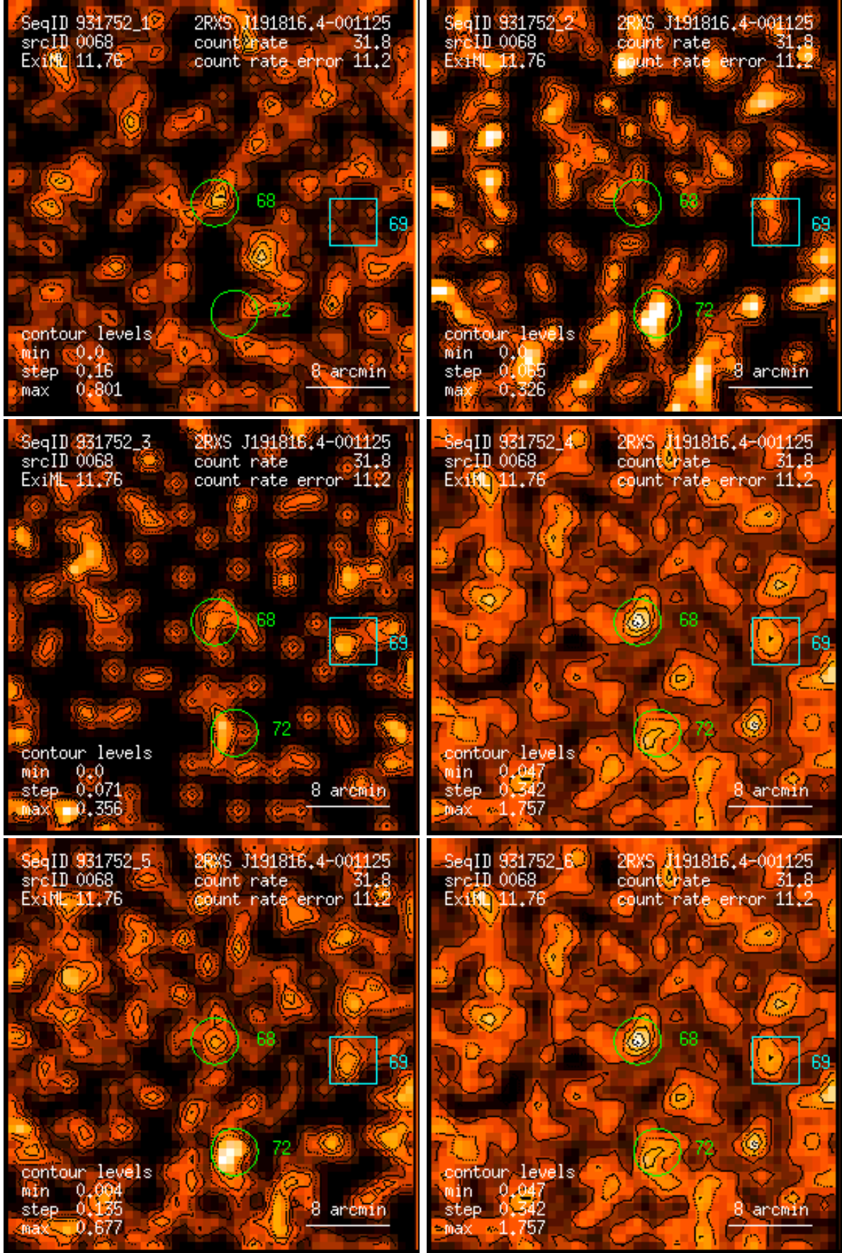
Figure 68: RASS 931752: detection 0068: band rate images, Gaussian filter: (1) PSPC channels 11 – 41, (2) 52 – 90, (3) 91 – 201, (4) 11 – 235, (5) 52 – 201, (6) 11 – 201. Broad band rates in counts/ks. Band rate contour levels in counts/ks/arcmin 2 .
