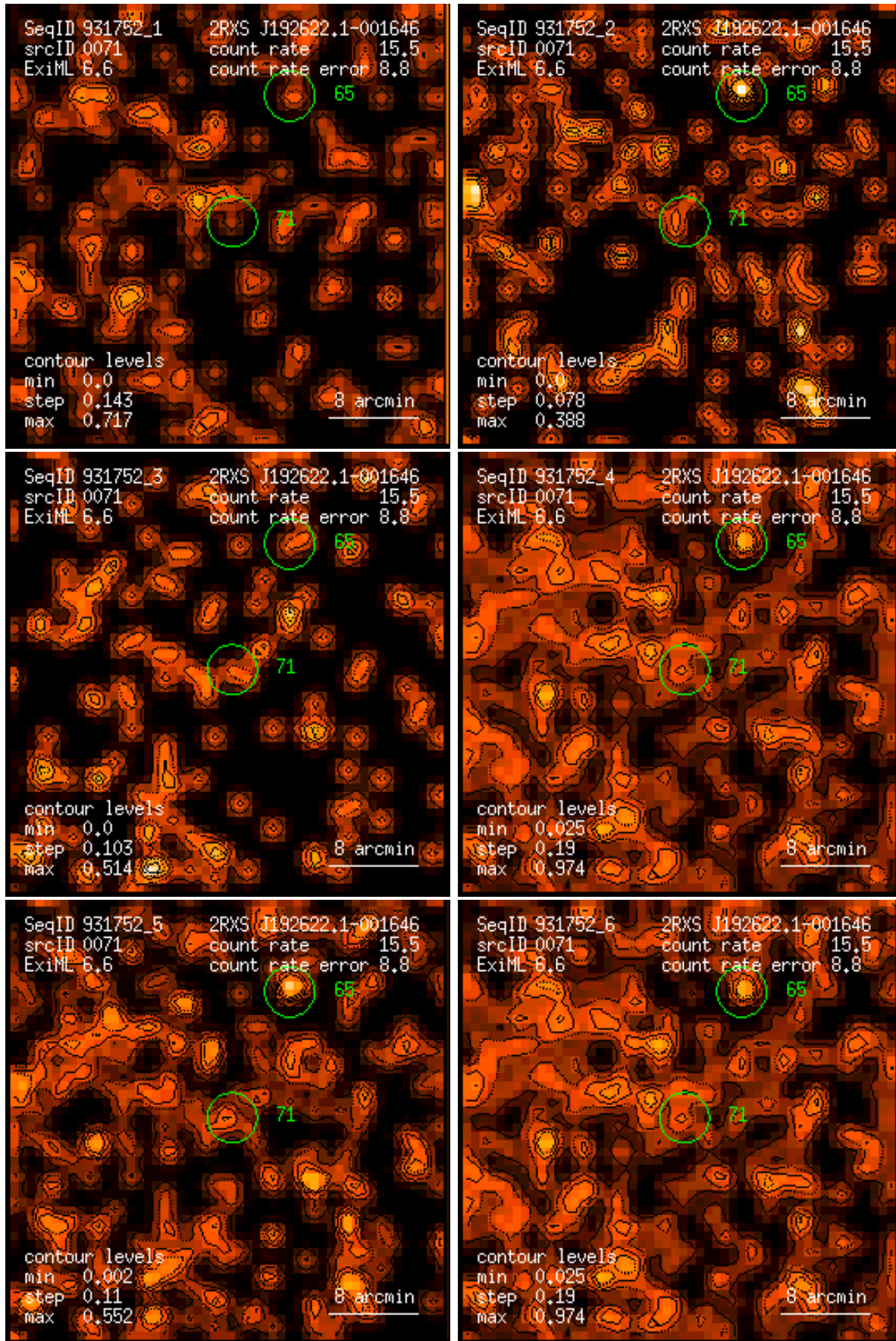
Figure 71: RASS 931752: detection 0071: band rate images, Gaussian filter: (1) PSPC channels 11 – 41, (2) 52 – 90, (3) 91 – 201, (4) 11 – 235, (5) 52 – 201, (6) 11 – 201. Broad band rates in counts/ks. Band rate contour levels in counts/ks/arcmin 2 .
