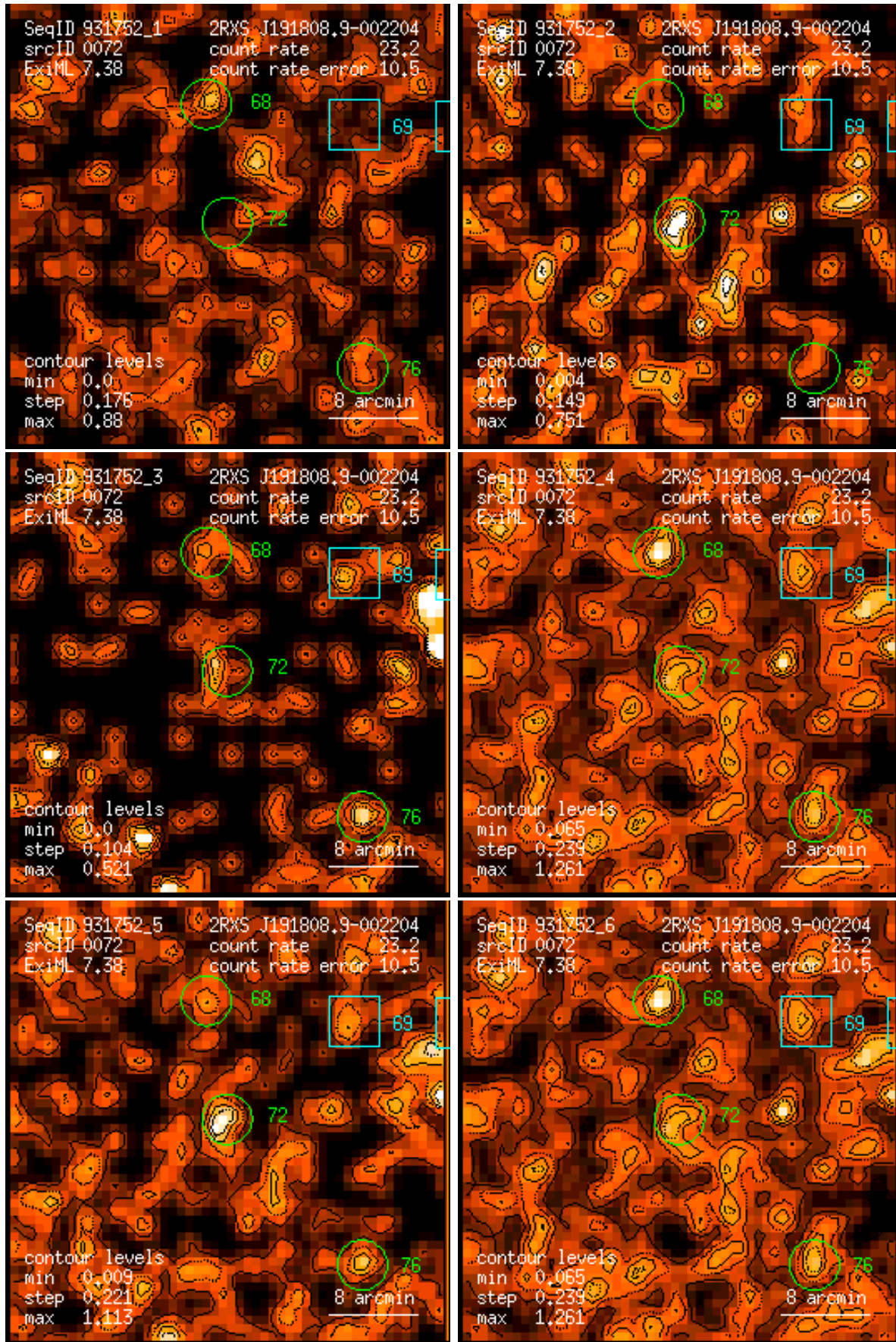
Figure 72: RASS 931752: detection 0072: band rate images, Gaussian filter: (1) PSPC channels 11 – 41, (2) 52 – 90, (3) 91 – 201, (4) 11 – 235, (5) 52 – 201, (6) 11 – 201. Broad band rates in counts/ks. Band rate contour levels in counts/ks/arcmin 2 .
