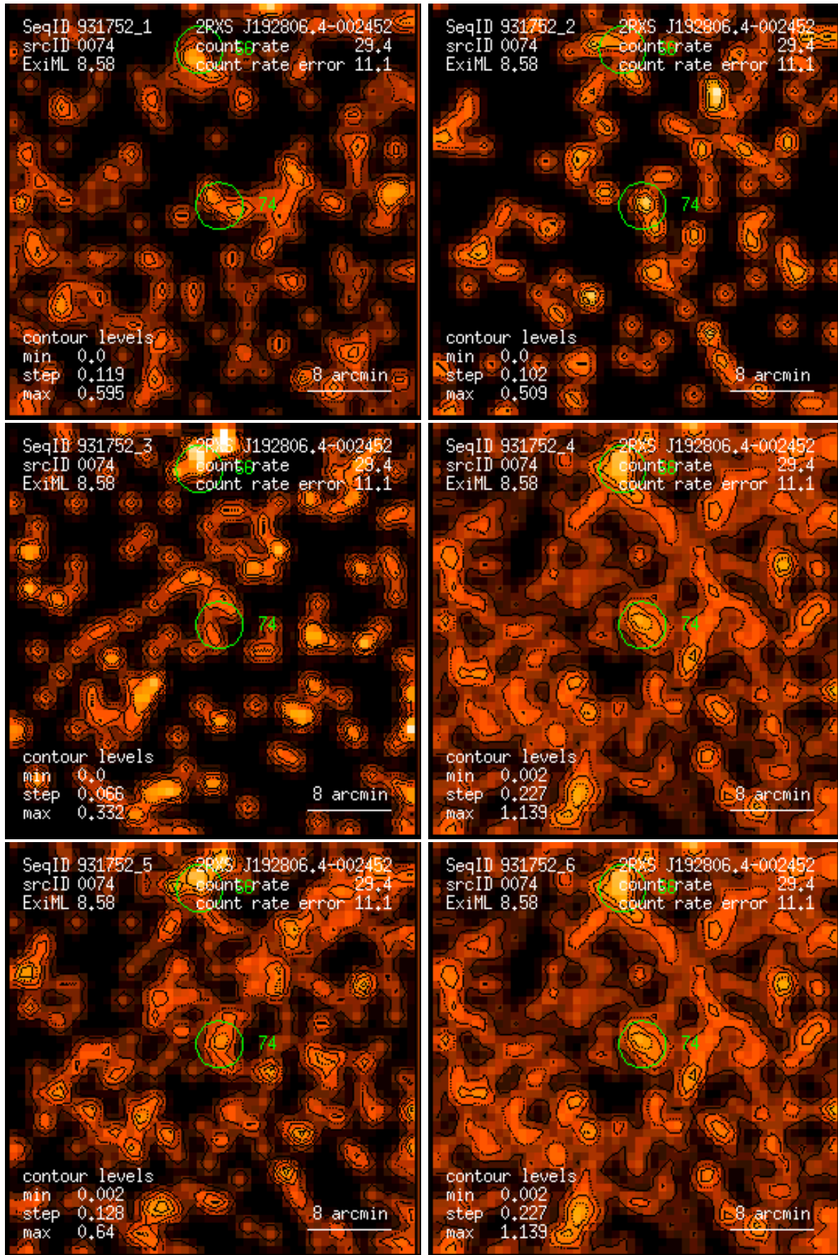
Figure 74: RASS 931752: detection 0074: band rate images, Gaussian filter: (1) PSPC channels 11 – 41, (2) 52 – 90, (3) 91 – 201, (4) 11 – 235, (5) 52 – 201, (6) 11 – 201. Broad band rates in counts/ks. Band rate contour levels in counts/ks/arcmin 2 .
