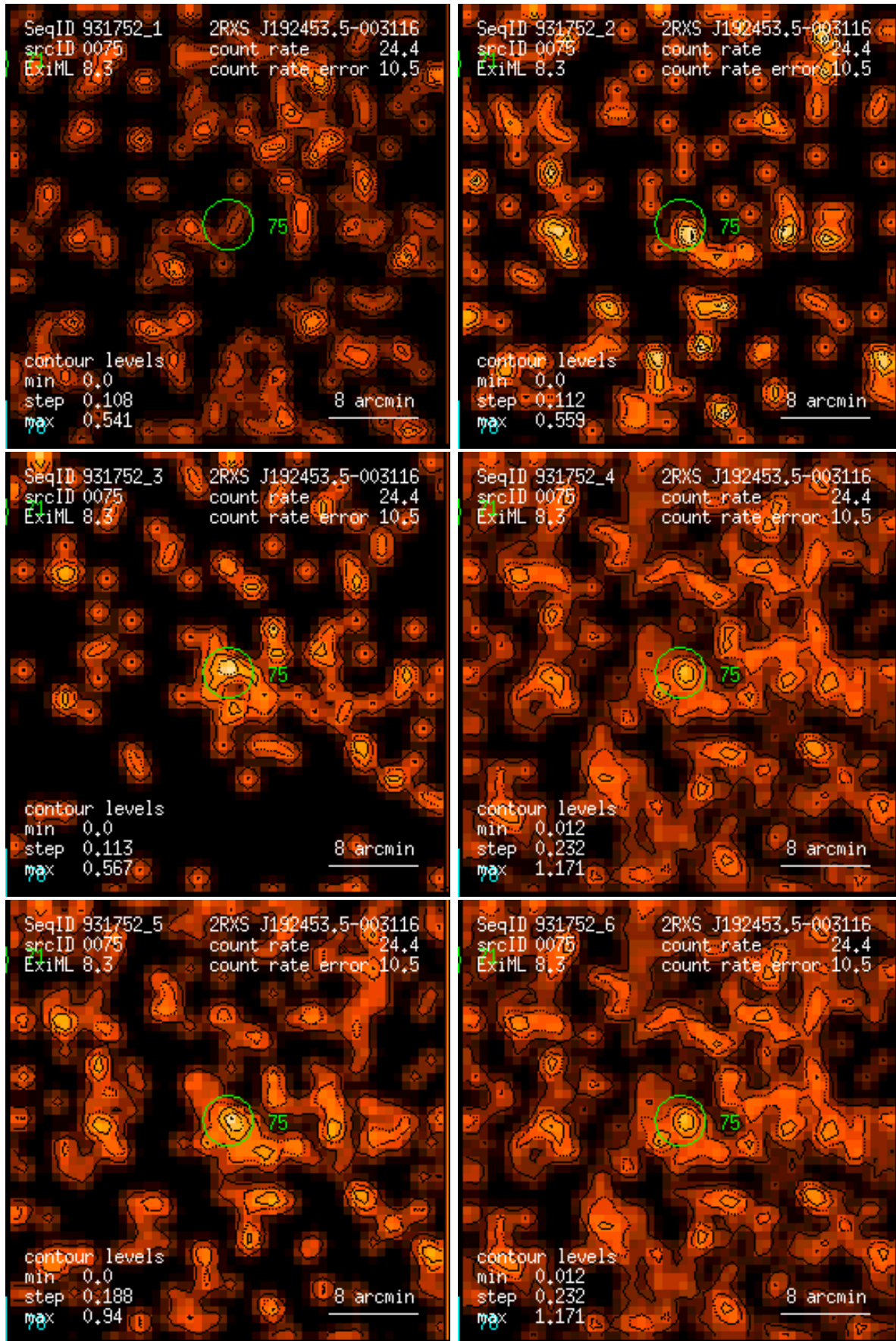
Figure 75: RASS 931752: detection 0075: band rate images, Gaussian filter: (1) PSPC channels 11 – 41, (2) 52 – 90, (3) 91 – 201, (4) 11 – 235, (5) 52 – 201, (6) 11 – 201. Broad band rates in counts/ks. Band rate contour levels in counts/ks/arcmin 2 .
