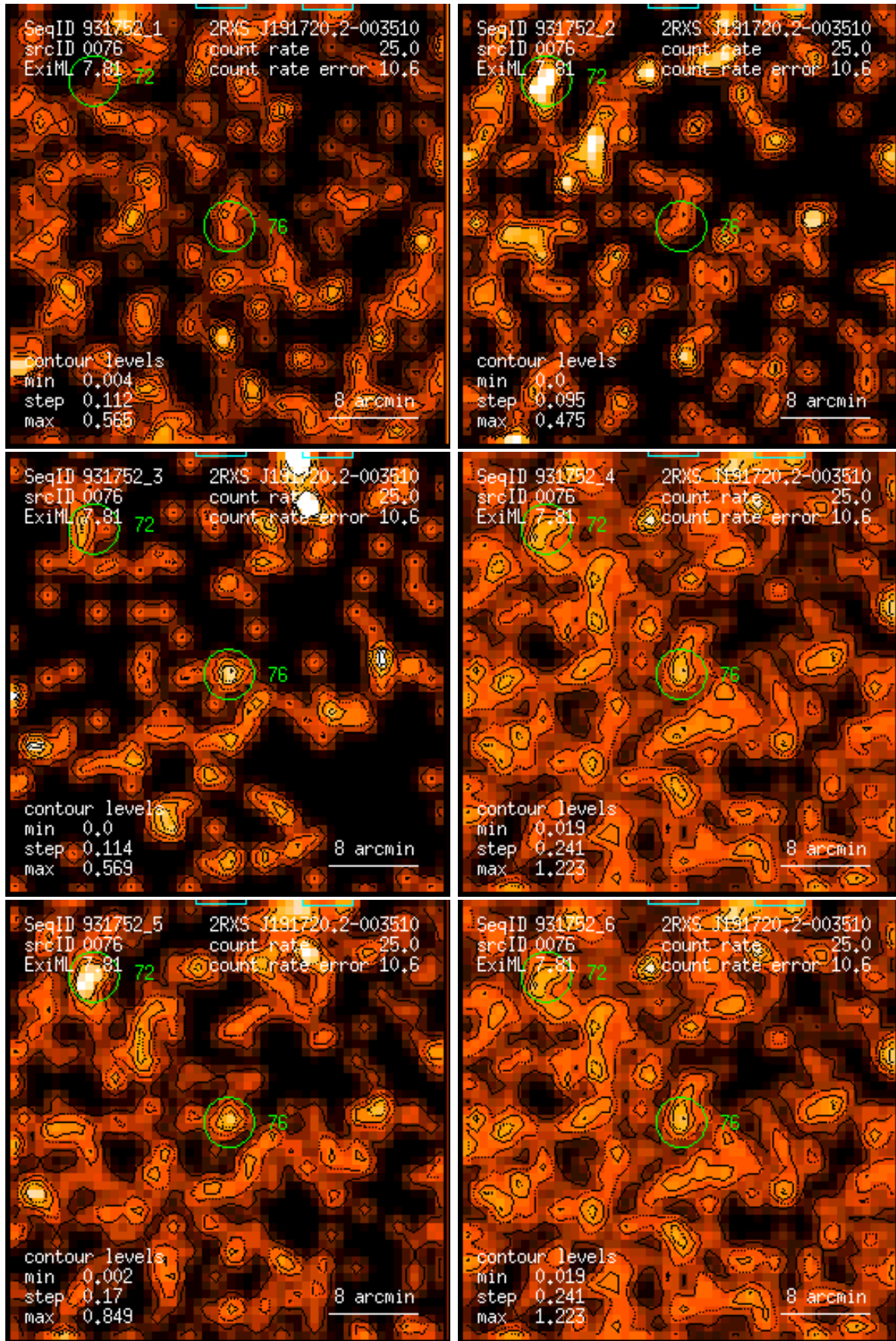
Figure 76: RASS 931752: detection 0076: band rate images, Gaussian filter: (1) PSPC channels 11 – 41, (2) 52 – 90, (3) 91 – 201, (4) 11 – 235, (5) 52 – 201, (6) 11 – 201. Broad band rates in counts/ks. Band rate contour levels in counts/ks/arcmin 2 .
