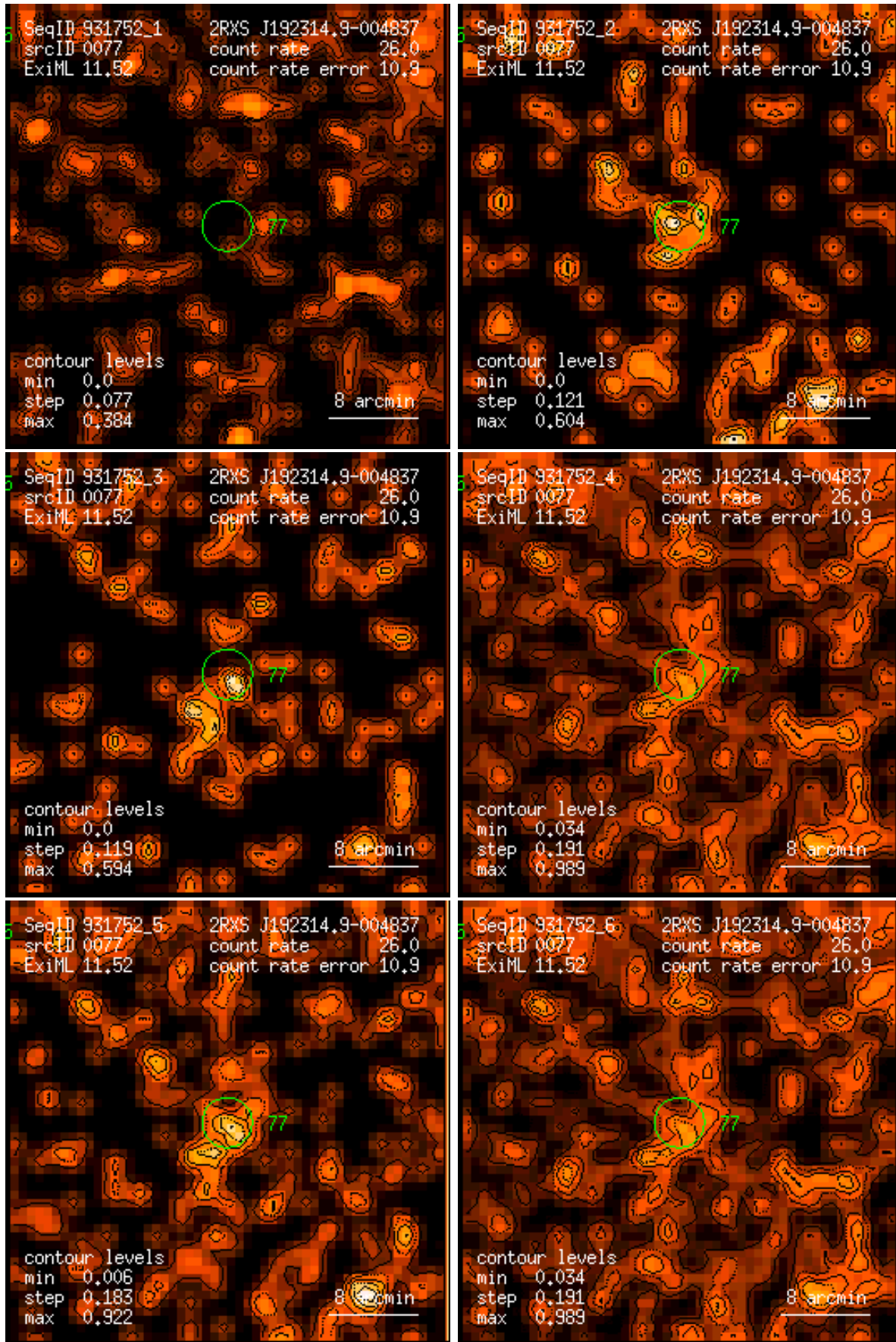
Figure 77: RASS 931752: detection 0077: band rate images, Gaussian filter: (1) PSPC channels 11 – 41, (2) 52 – 90, (3) 91 – 201, (4) 11 – 235, (5) 52 – 201, (6) 11 – 201. Broad band rates in counts/ks. Band rate contour levels in counts/ks/arcmin 2 .
