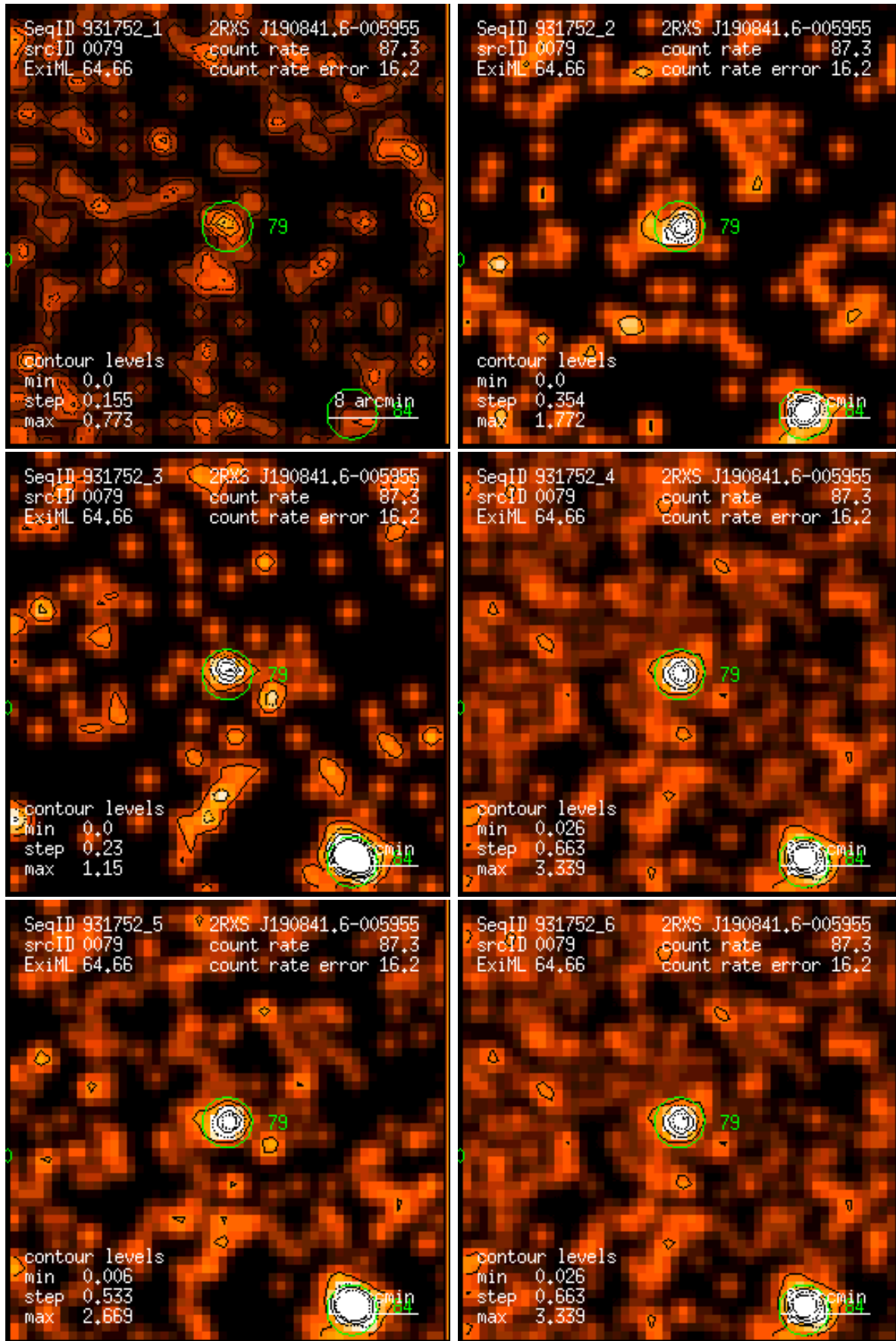
Figure 79: RASS 931752: detection 0079: band rate images, Gaussian filter: (1) PSPC channels 11 – 41, (2) 52 – 90, (3) 91 – 201, (4) 11 – 235, (5) 52 – 201, (6) 11 – 201. Broad band rates in counts/ks. Band rate contour levels in counts/ks/arcmin 2 .
