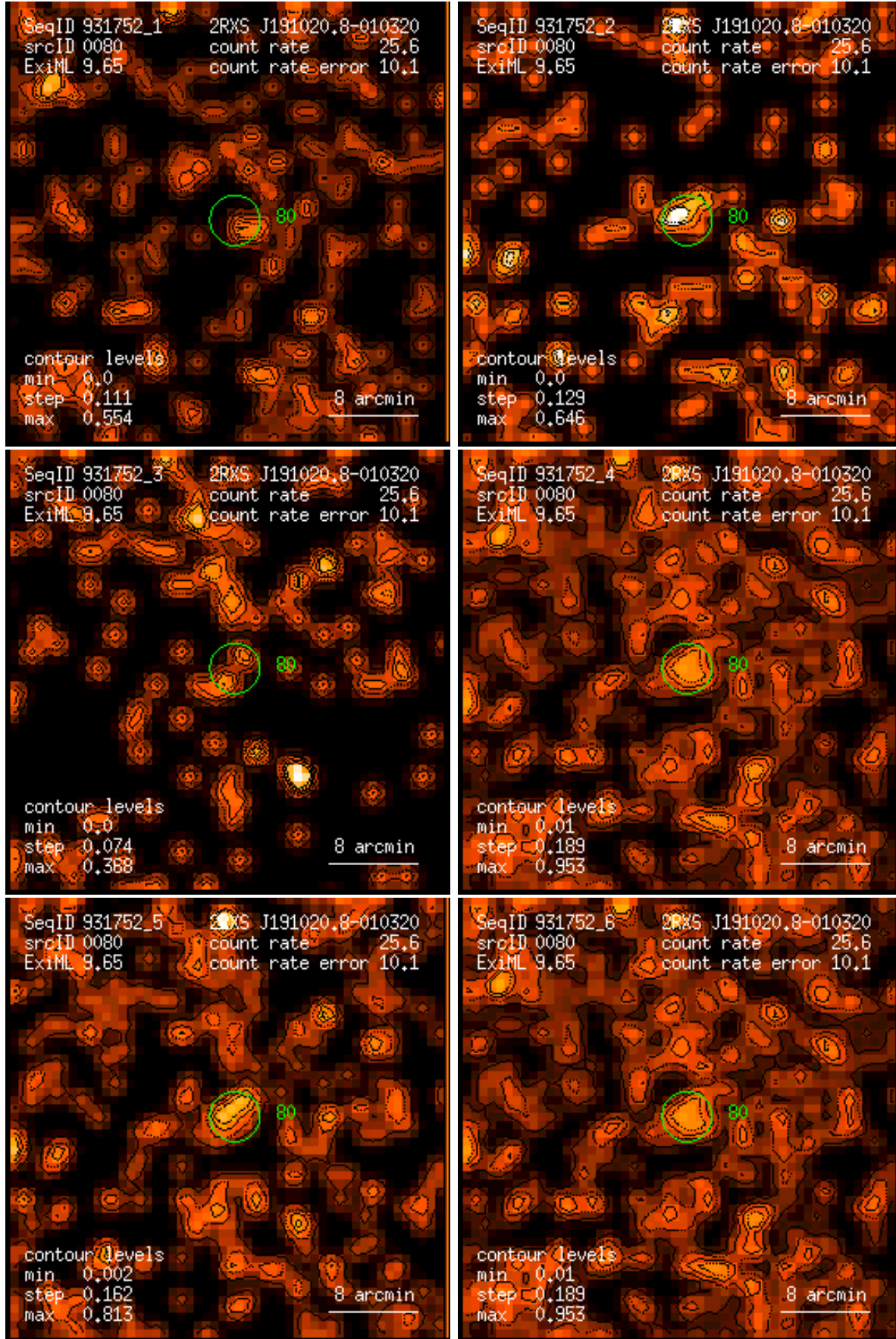
Figure 80: RASS 931752: detection 0080: band rate images, Gaussian filter: (1) PSPC channels 11 – 41, (2) 52 – 90, (3) 91 – 201, (4) 11 – 235, (5) 52 – 201, (6) 11 – 201. Broad band rates in counts/ks. Band rate contour levels in counts/ks/arcmin 2 .
