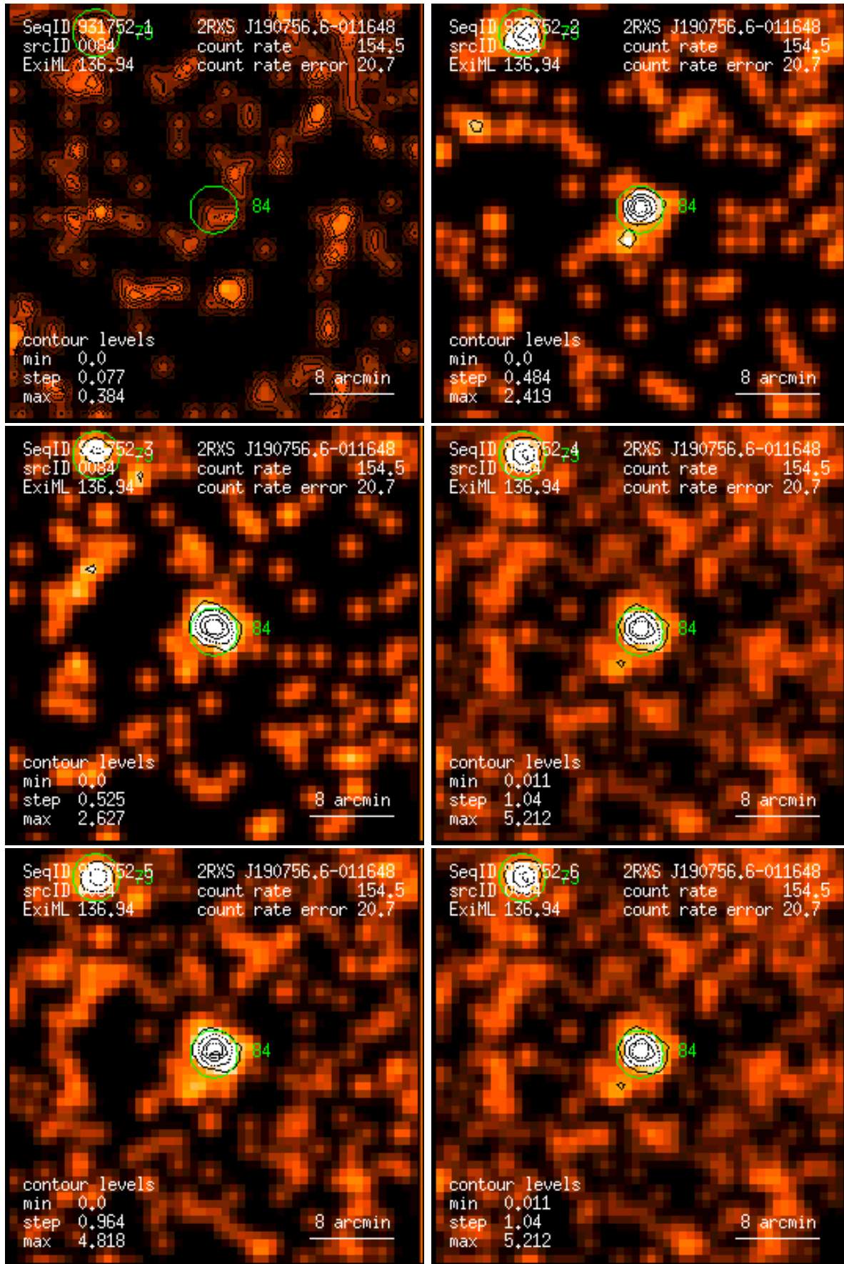
Figure 84: RASS 931752: detection 0084: band rate images, Gaussian filter: (1) PSPC channels 11 – 41, (2) 52 – 90, (3) 91 – 201, (4) 11 – 235, (5) 52 – 201, (6) 11 – 201. Broad band rates in counts/ks. Band rate contour levels in counts/ks/arcmin 2 .
