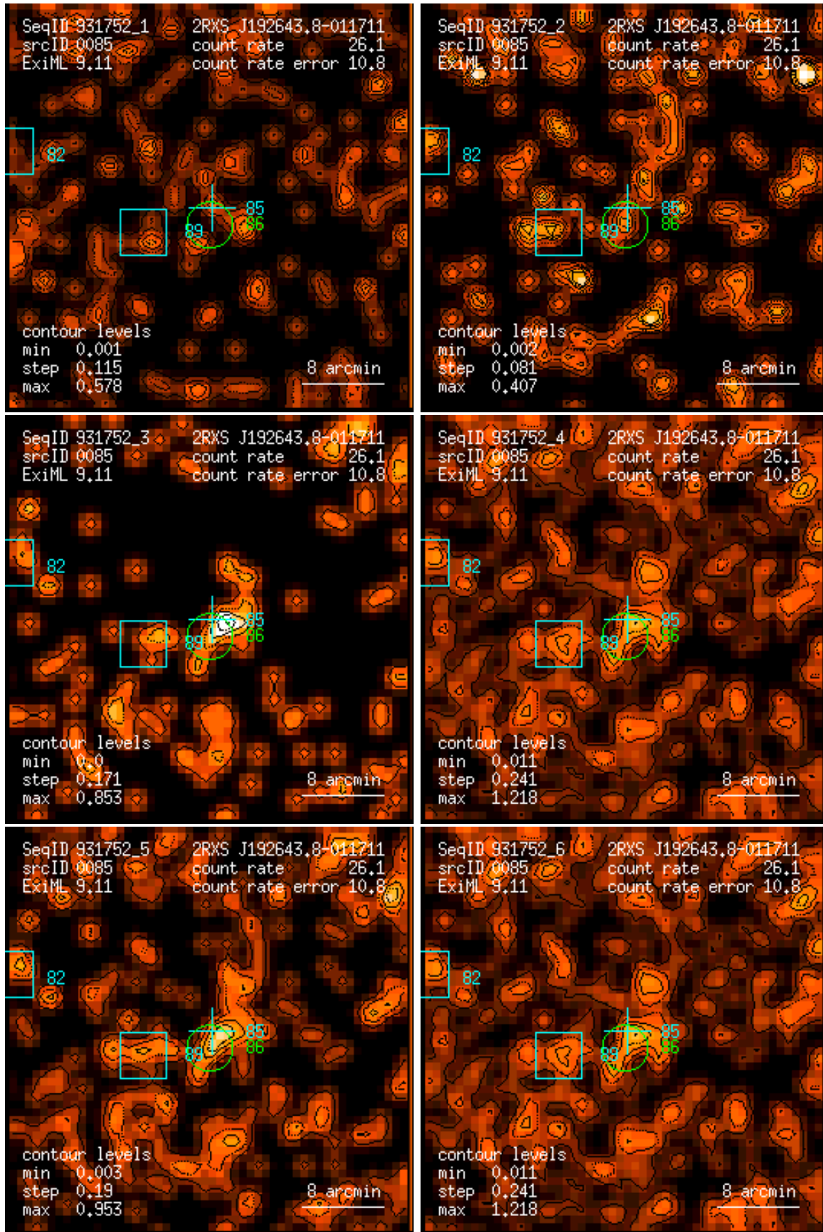
Figure 85: RASS 931752: detection 0085: band rate images, Gaussian filter: (1) PSPC channels 11 – 41, (2) 52 – 90, (3) 91 – 201, (4) 11 – 235, (5) 52 – 201, (6) 11 – 201. Broad band rates in counts/ks. Band rate contour levels in counts/ks/arcmin 2 .
