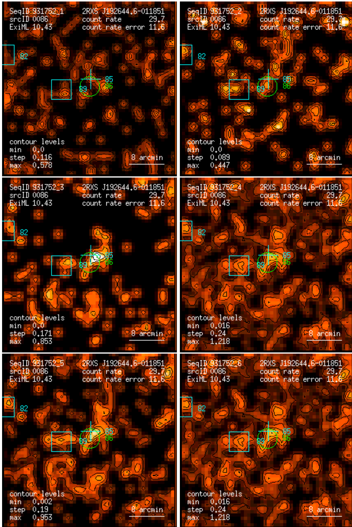
Figure 86: RASS 931752: detection 0086: band rate images, Gaussian filter: (1) PSPC channels 11 – 41, (2) 52 – 90, (3) 91 – 201, (4) 11 – 235, (5) 52 – 201, (6) 11 – 201. Broad band rates in counts/ks. Band rate contour levels in counts/ks/arcmin 2 .
