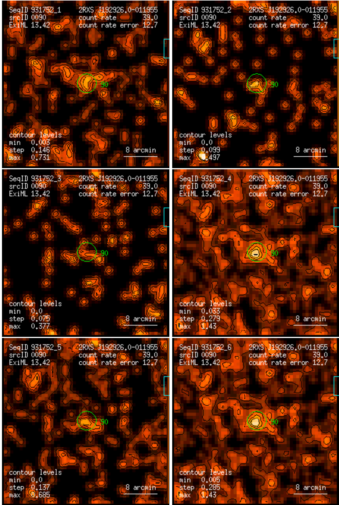
Figure 90: RASS 931752: detection 0090: band rate images, Gaussian filter: (1) PSPC channels 11 – 41, (2) 52 – 90, (3) 91 – 201, (4) 11 – 235, (5) 52 – 201, (6) 11 – 201. Broad band rates in counts/ks. Band rate contour levels in counts/ks/arcmin 2 .
