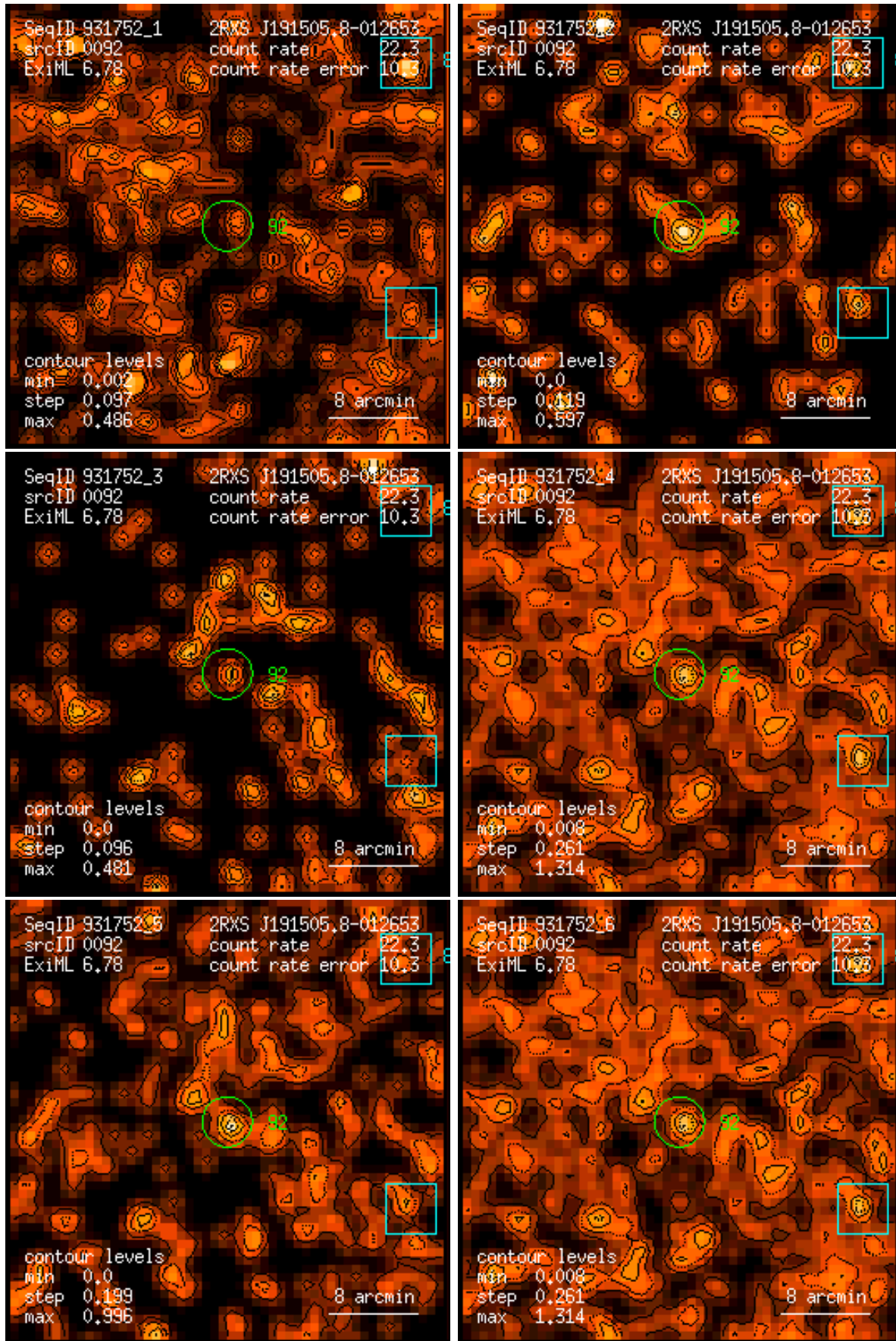
Figure 92: RASS 931752: detection 0092: band rate images, Gaussian filter: (1) PSPC channels 11 – 41, (2) 52 – 90, (3) 91 – 201, (4) 11 – 235, (5) 52 – 201, (6) 11 – 201. Broad band rates in counts/ks. Band rate contour levels in counts/ks/arcmin 2 .
