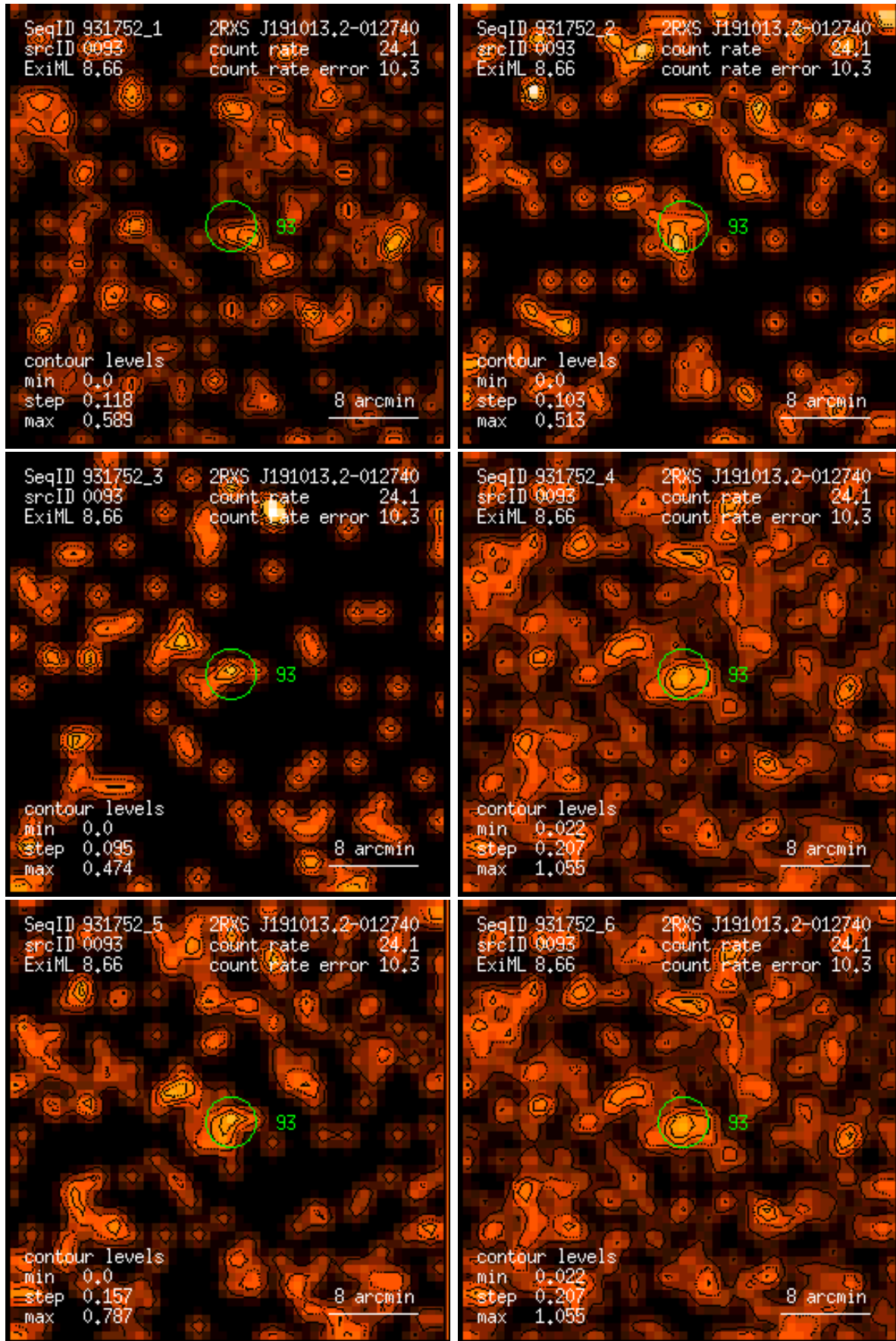
Figure 93: RASS 931752: detection 0093: band rate images, Gaussian filter: (1) PSPC channels 11 – 41, (2) 52 – 90, (3) 91 – 201, (4) 11 – 235, (5) 52 – 201, (6) 11 – 201. Broad band rates in counts/ks. Band rate contour levels in counts/ks/arcmin 2 .
