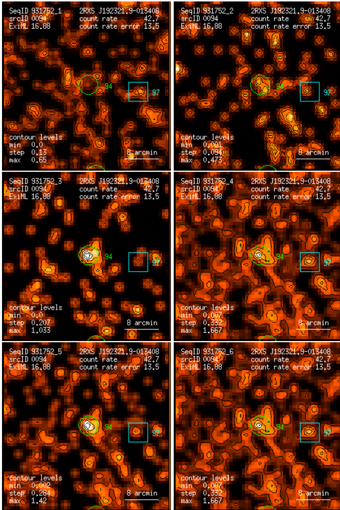
Figure 94: RASS 931752: detection 0094: band rate images, Gaussian filter: (1) PSPC channels 11 – 41, (2) 52 – 90, (3) 91 – 201, (4) 11 – 235, (5) 52 – 201, (6) 11 – 201. Broad band rates in counts/ks. Band rate contour levels in counts/ks/arcmin 2 .
