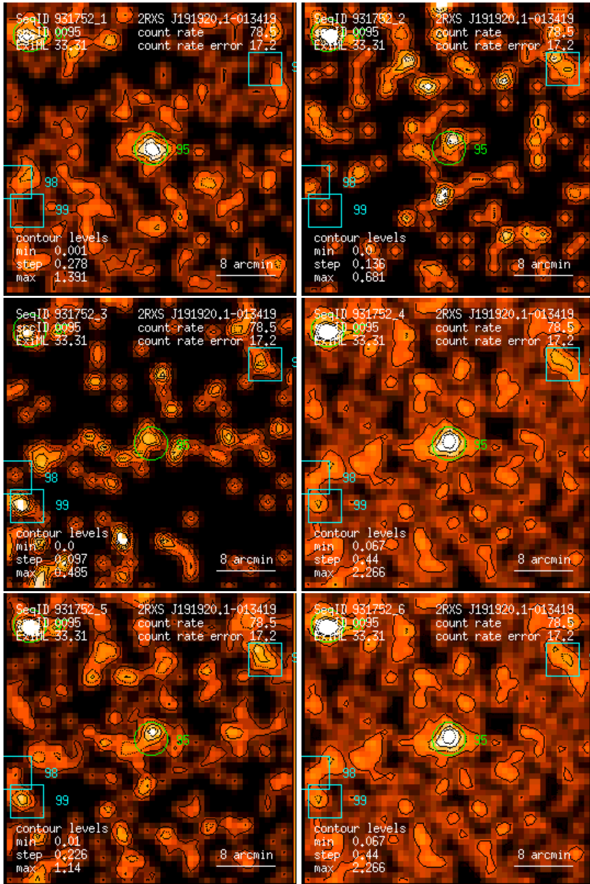
Figure 95: RASS 931752: detection 0095: band rate images, Gaussian filter: (1) PSPC channels 11 – 41, (2) 52 – 90, (3) 91 – 201, (4) 11 – 235, (5) 52 – 201, (6) 11 – 201. Broad band rates in counts/ks. Band rate contour levels in counts/ks/arcmin 2 .
