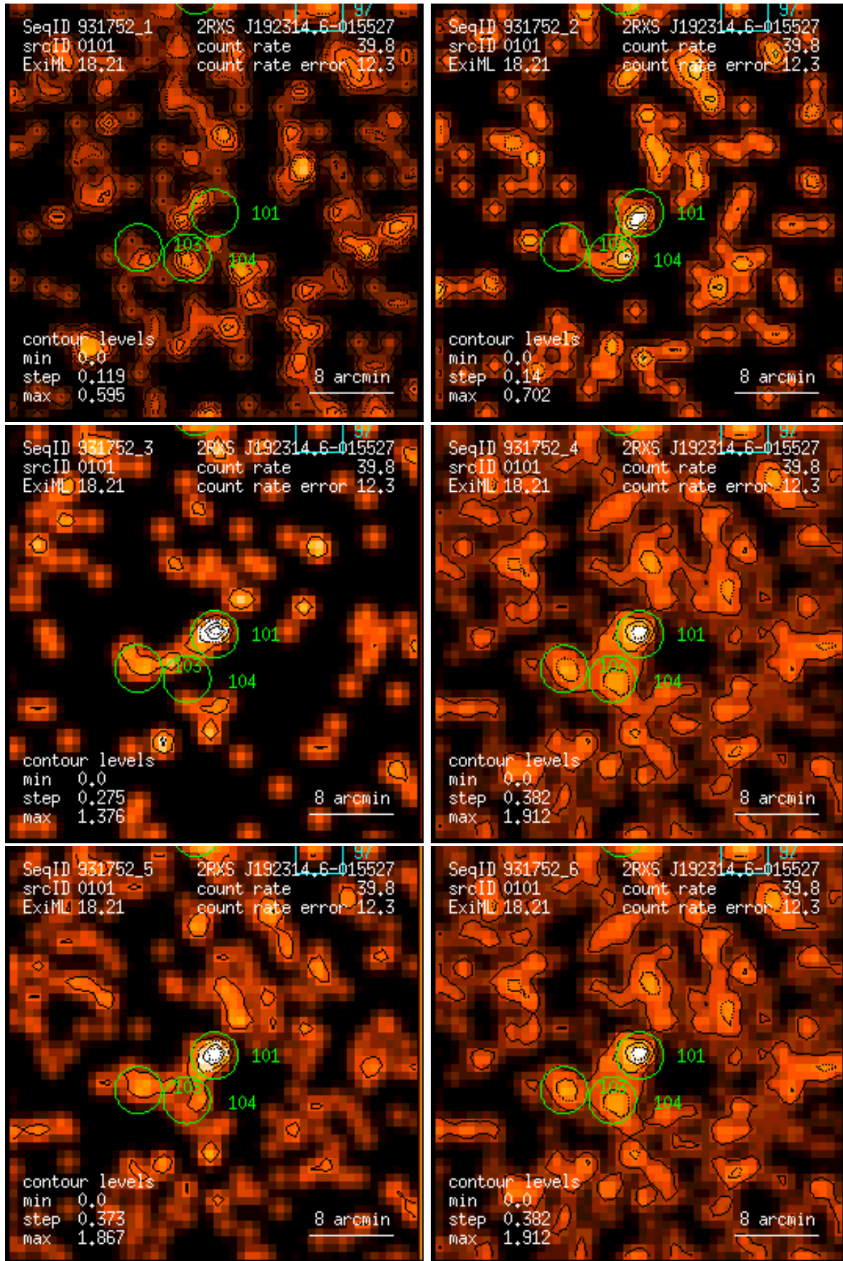
Figure 101: RASS 931752: detection 0101: band rate images, Gaussian filter: (1) PSPC channels 11 – 41, (2) 52 – 90, (3) 91 – 201, (4) 11 – 235, (5) 52 – 201, (6) 11 – 201. Broad band rates in counts/ks. Band rate contour levels in counts/ks/arcmin 2 .
