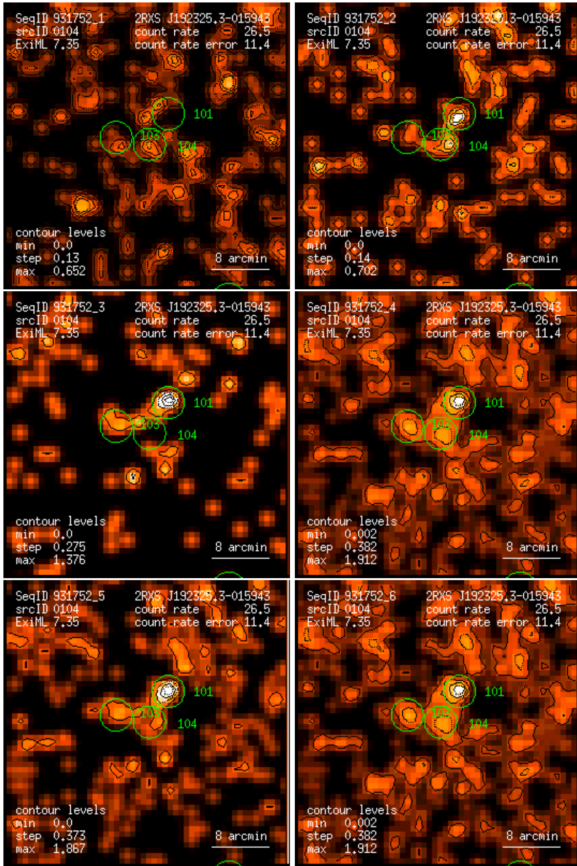
Figure 104: RASS 931752: detection 0104: band rate images, Gaussian filter: (1) PSPC channels 11 – 41, (2) 52 – 90, (3) 91 – 201, (4) 11 – 235, (5) 52 – 201, (6) 11 – 201. Broad band rates in counts/ks. Band rate contour levels in counts/ks/arcmin 2 .
