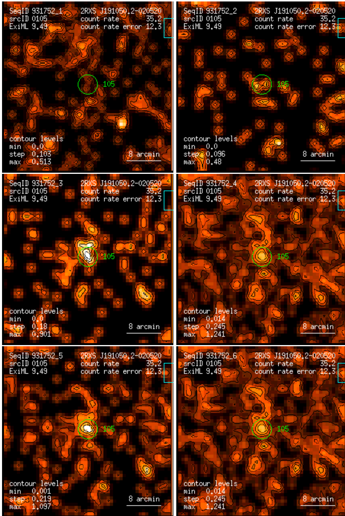
Figure 105: RASS 931752: detection 0105: band rate images, Gaussian filter: (1) PSPC channels 11 – 41, (2) 52 – 90, (3) 91 – 201, (4) 11 – 235, (5) 52 – 201, (6) 11 – 201. Broad band rates in counts/ks. Band rate contour levels in counts/ks/arcmin 2 .
