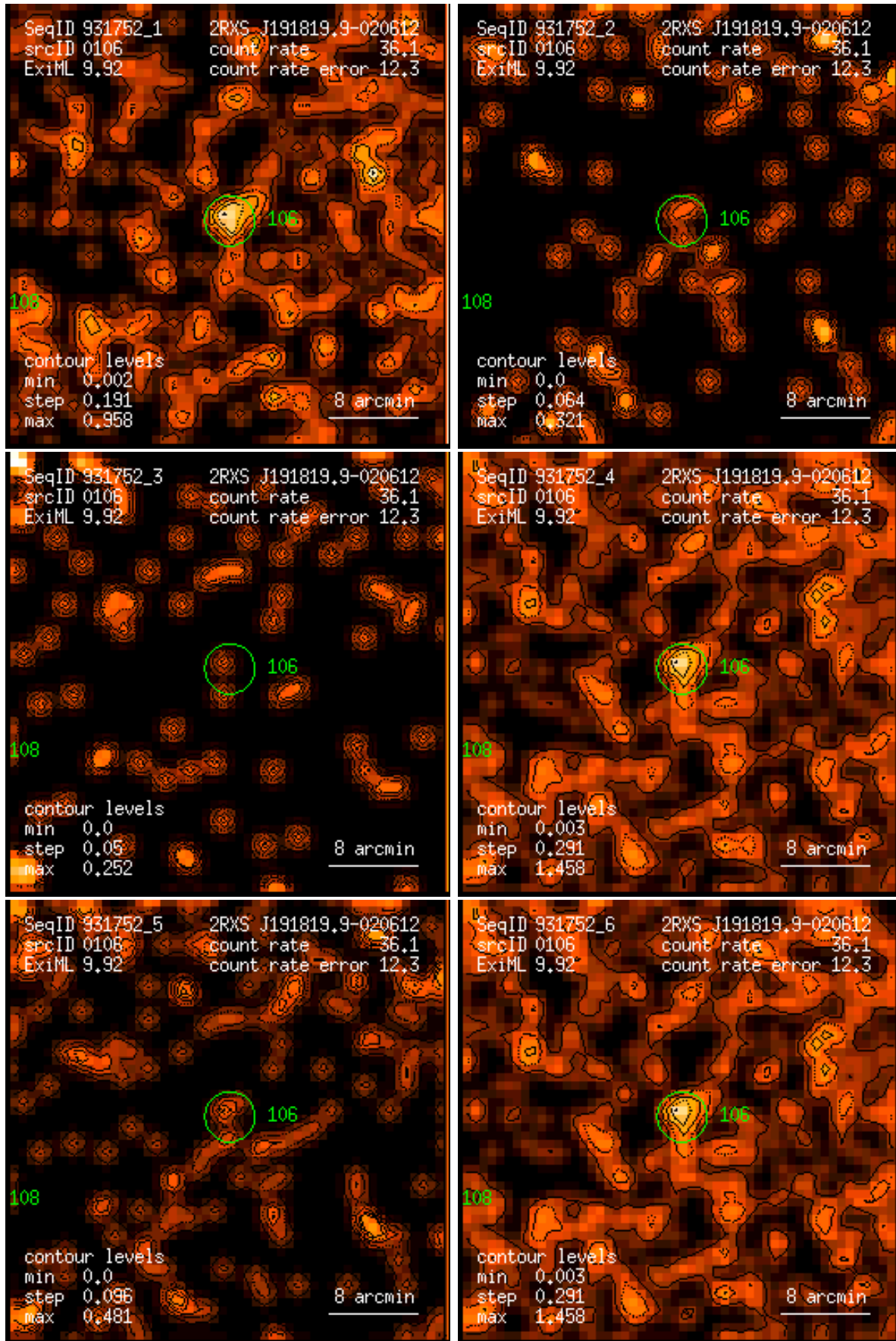
Figure 106: RASS 931752: detection 0106: band rate images, Gaussian filter: (1) PSPC channels 11 – 41, (2) 52 – 90, (3) 91 – 201, (4) 11 – 235, (5) 52 – 201, (6) 11 – 201. Broad band rates in counts/ks. Band rate contour levels in counts/ks/arcmin 2 .
