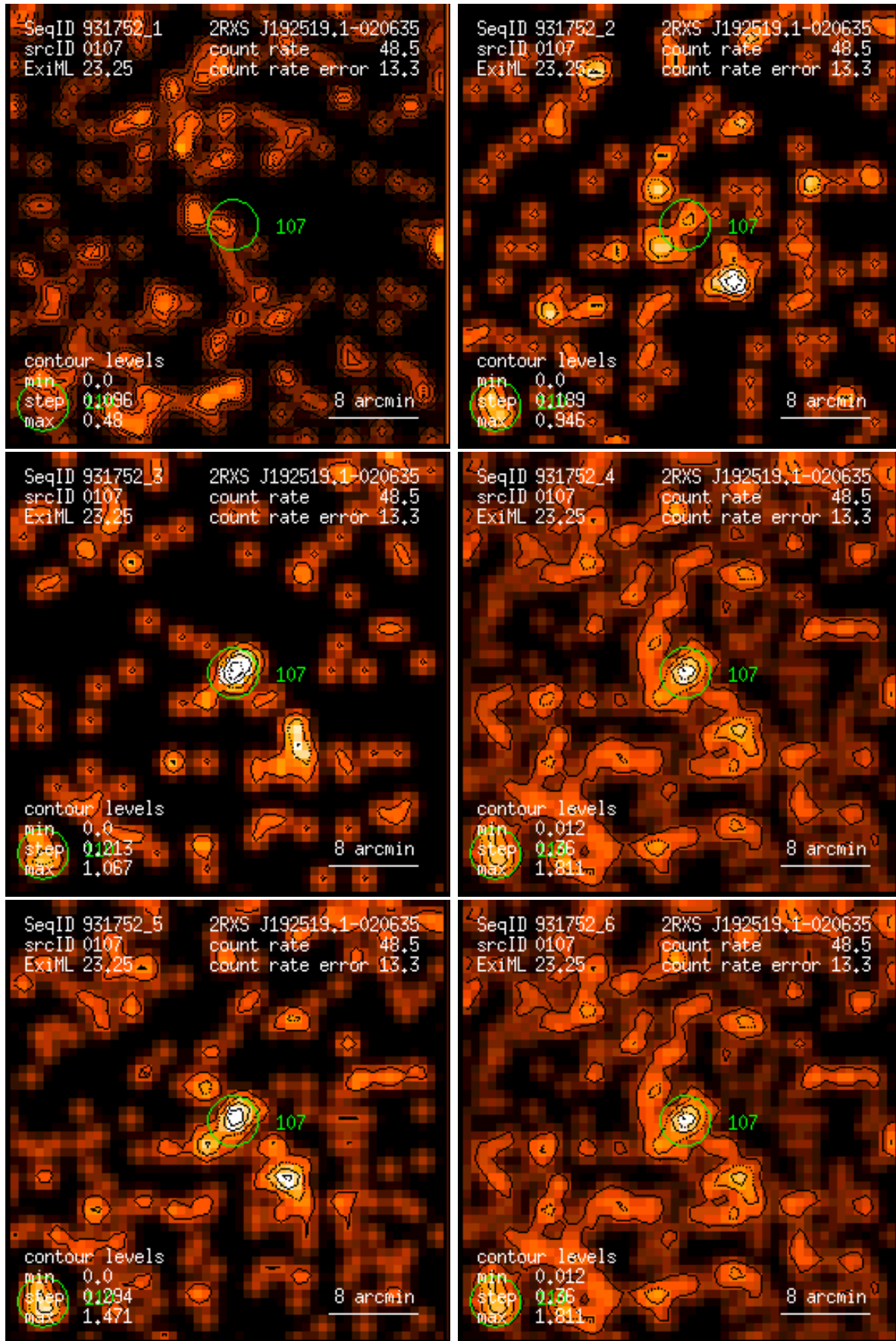
Figure 107: RASS 931752: detection 0107: band rate images, Gaussian filter: (1) PSPC channels 11 – 41, (2) 52 – 90, (3) 91 – 201, (4) 11 – 235, (5) 52 – 201, (6) 11 – 201. Broad band rates in counts/ks. Band rate contour levels in counts/ks/arcmin 2 .
