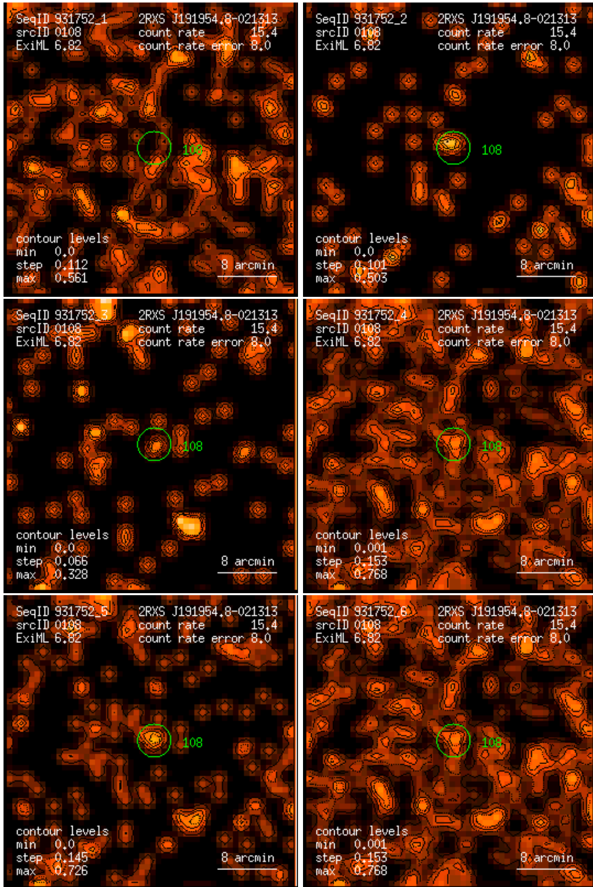
Figure 108: RASS 931752: detection 0108: band rate images, Gaussian filter: (1) PSPC channels 11 – 41, (2) 52 – 90, (3) 91 – 201, (4) 11 – 235, (5) 52 – 201, (6) 11 – 201. Broad band rates in counts/ks. Band rate contour levels in counts/ks/arcmin 2 .
