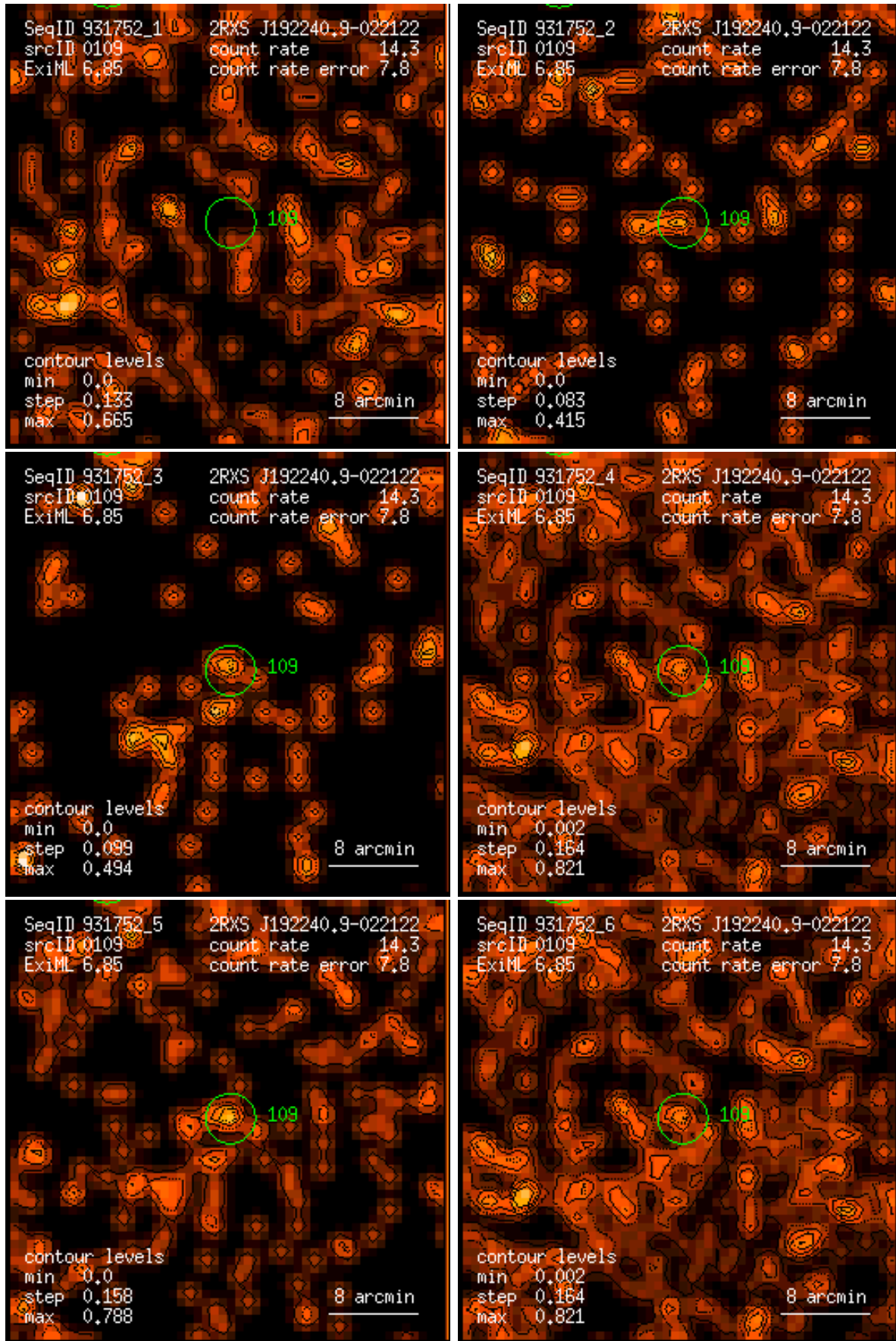
Figure 109: RASS 931752: detection 0109: band rate images, Gaussian filter: (1) PSPC channels 11 – 41, (2) 52 – 90, (3) 91 – 201, (4) 11 – 235, (5) 52 – 201, (6) 11 – 201. Broad band rates in counts/ks. Band rate contour levels in counts/ks/arcmin 2 .
