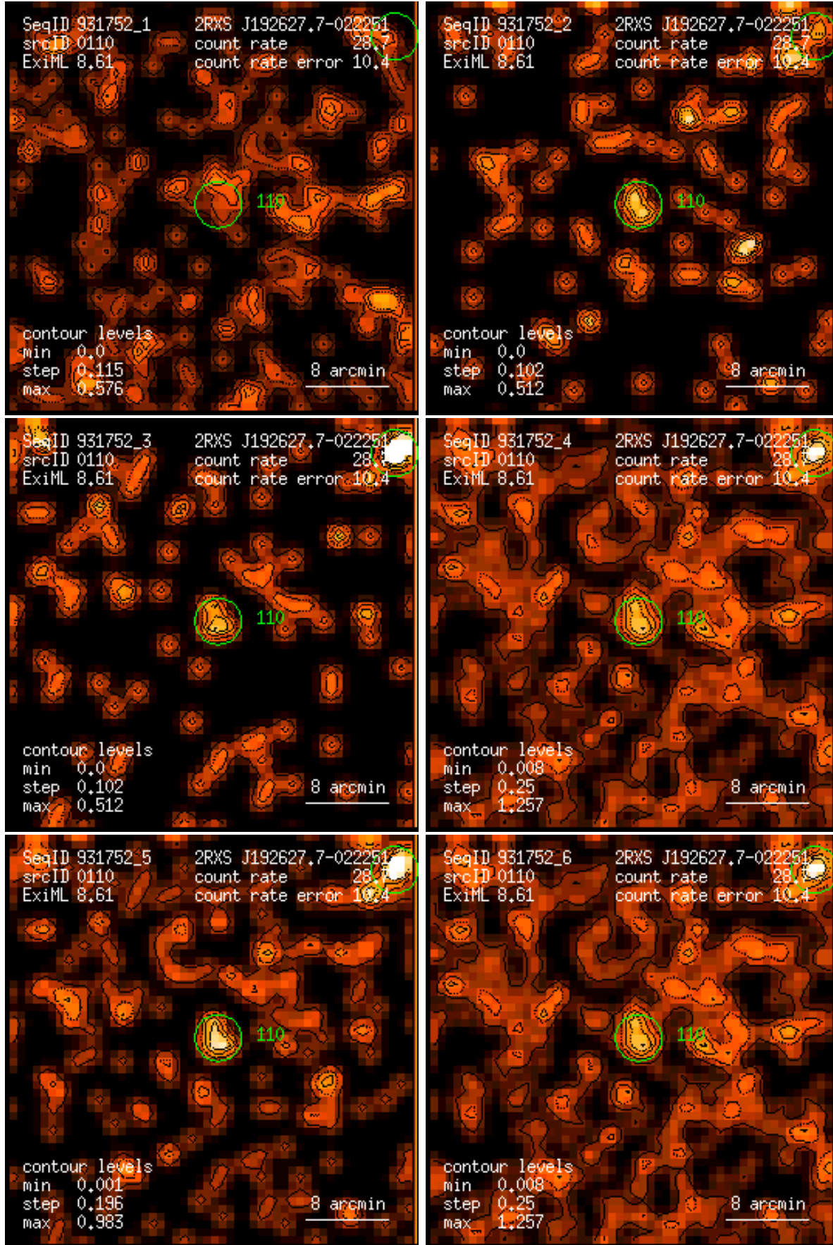
Figure 110: RASS 931752: detection 0110: band rate images, Gaussian filter: (1) PSPC channels 11 – 41, (2) 52 – 90, (3) 91 – 201, (4) 11 – 235, (5) 52 – 201, (6) 11 – 201. Broad band rates in counts/ks. Band rate contour levels in counts/ks/arcmin 2 .
