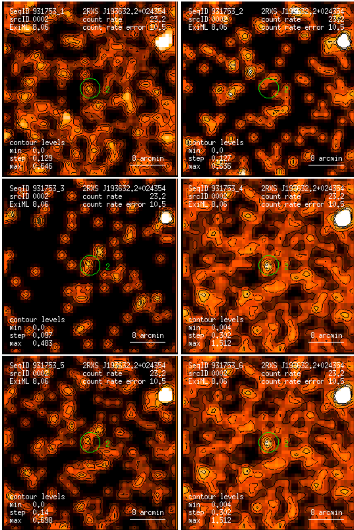
Figure 2: RASS 931753: detection 0002: band rate images, Gaussian filter: (1) PSPC channels 11 – 41, (2) 52 – 90, (3) 91 – 201, (4) 11 – 235, (5) 52 – 201, (6) 11 – 201. Broad band rates in counts/ks. Band rate contour levels in counts/ks/arcmin 2 .
