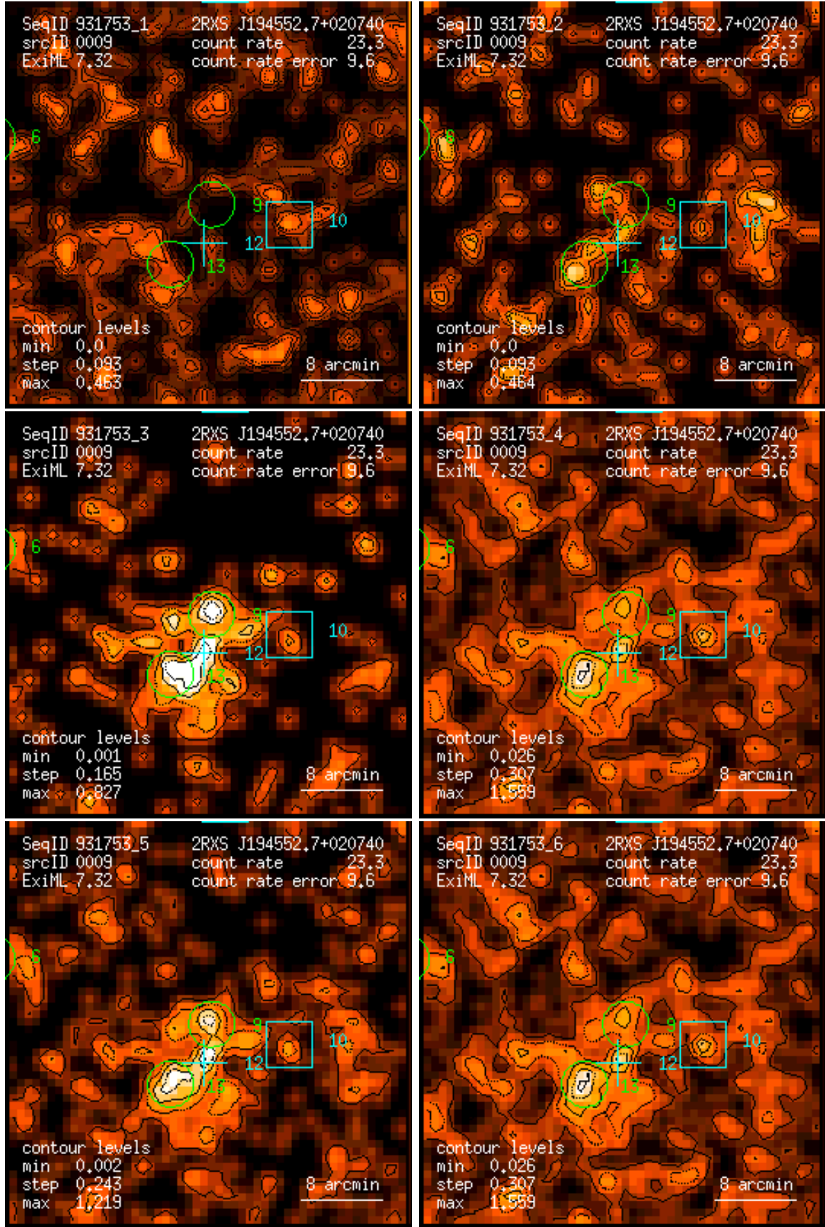
Figure 9: RASS 931753: detection 0009: band rate images, Gaussian filter: (1) PSPC channels 11 – 41, (2) 52 – 90, (3) 91 – 201, (4) 11 – 235, (5) 52 – 201, (6) 11 – 201. Broad band rates in counts/ks. Band rate contour levels in counts/ks/arcmin 2 .
