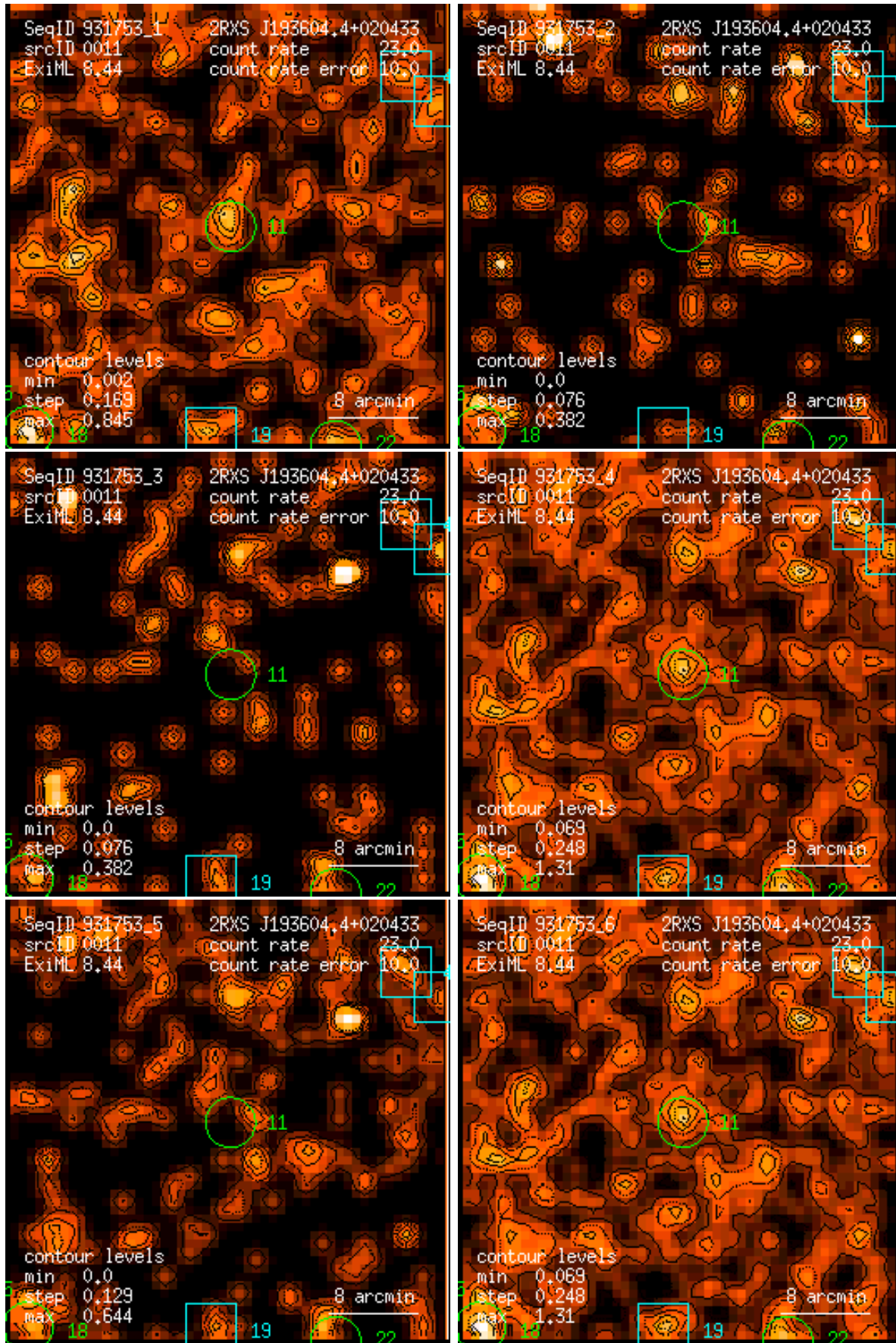
Figure 11: RASS 931753: detection 0011: band rate images, Gaussian filter: (1) PSPC channels 11 – 41, (2) 52 – 90, (3) 91 – 201, (4) 11 – 235, (5) 52 – 201, (6) 11 – 201. Broad band rates in counts/ks. Band rate contour levels in counts/ks/arcmin 2 .
