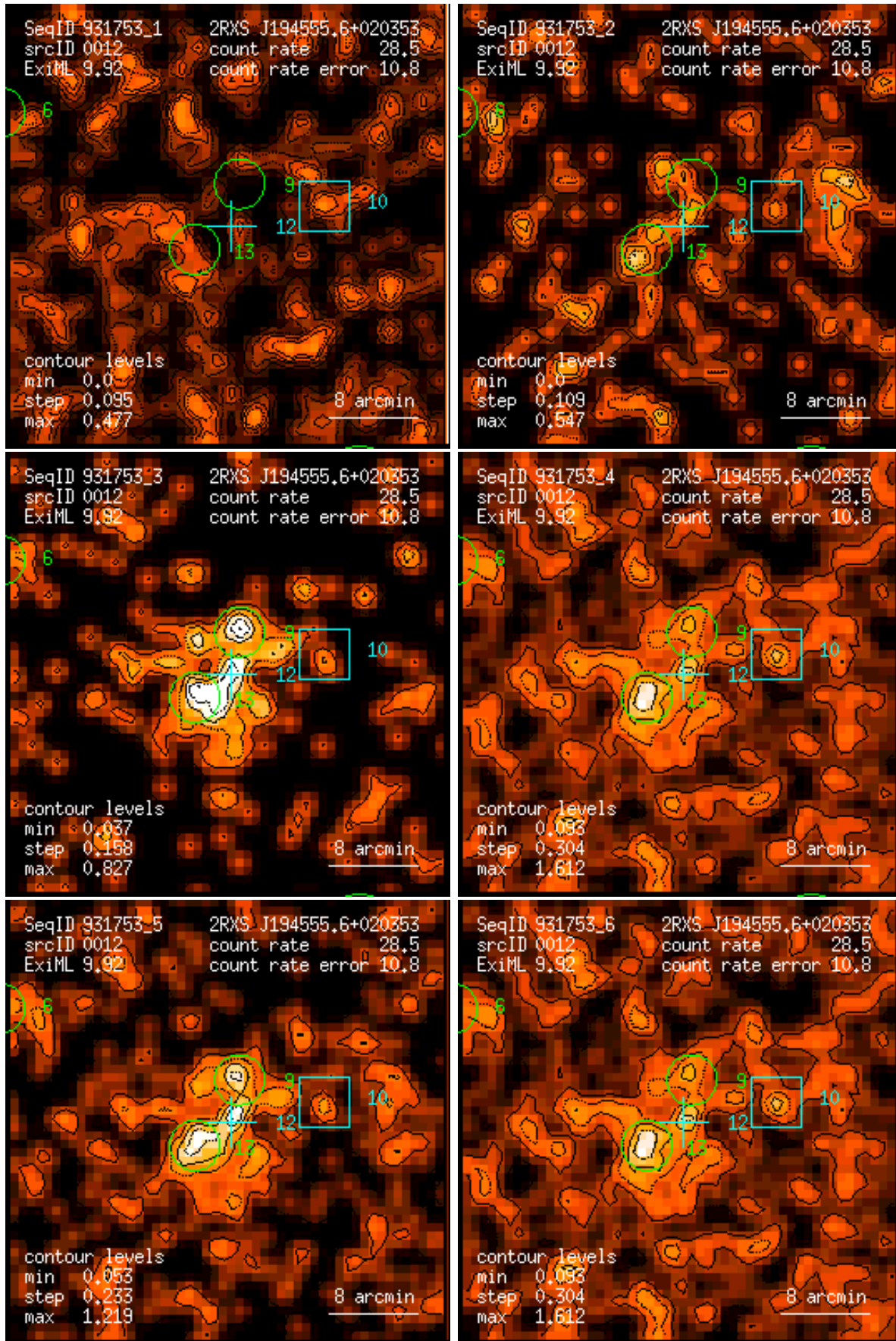
Figure 12: RASS 931753: detection 0012: band rate images, Gaussian filter: (1) PSPC channels 11 – 41, (2) 52 – 90, (3) 91 – 201, (4) 11 – 235, (5) 52 – 201, (6) 11 – 201. Broad band rates in counts/ks. Band rate contour levels in counts/ks/arcmin 2 .
