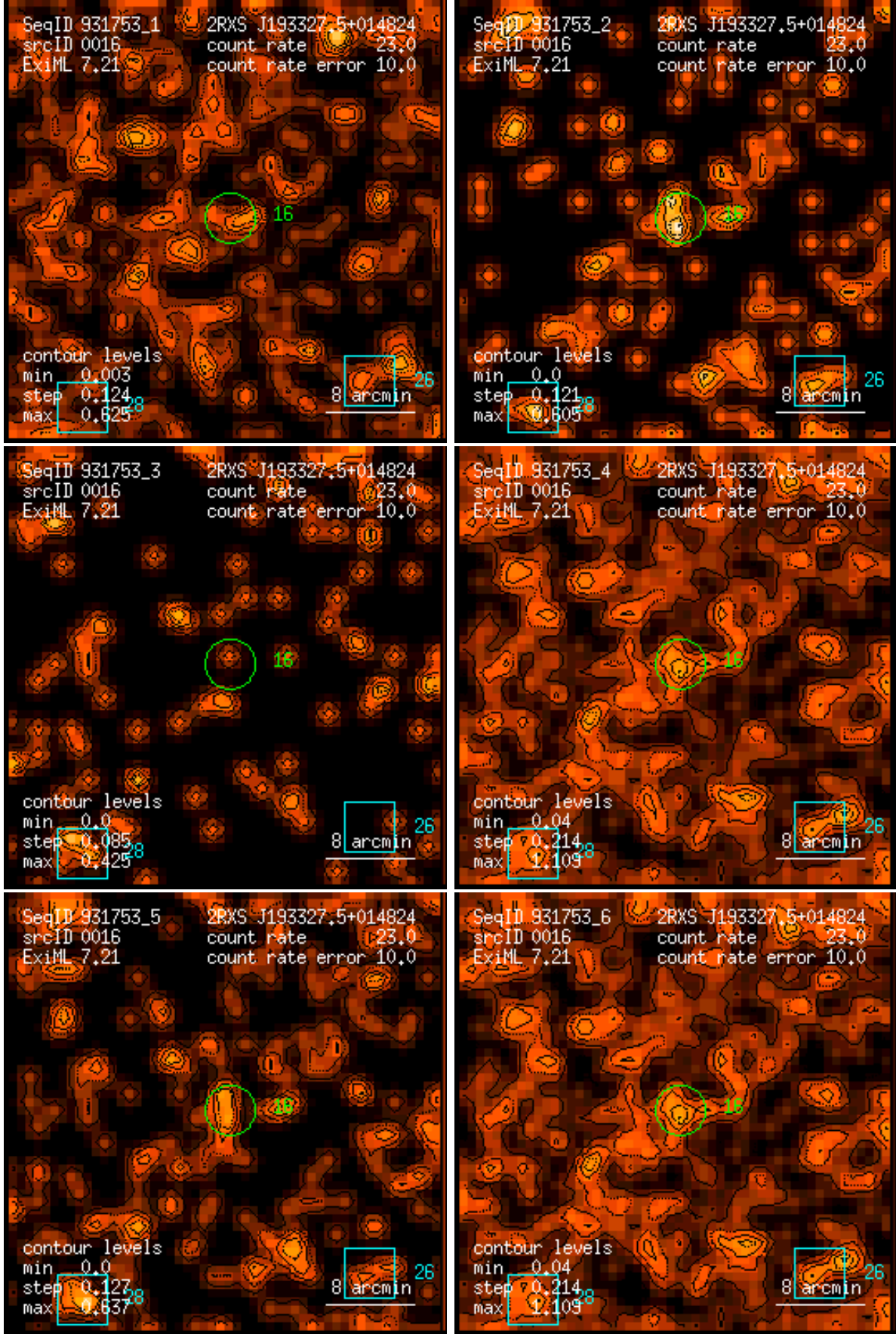
Figure 16: RASS 931753: detection 0016: band rate images, Gaussian filter: (1) PSPC channels 11 – 41, (2) 52 – 90, (3) 91 – 201, (4) 11 – 235, (5) 52 – 201, (6) 11 – 201. Broad band rates in counts/ks. Band rate contour levels in counts/ks/arcmin 2 .
