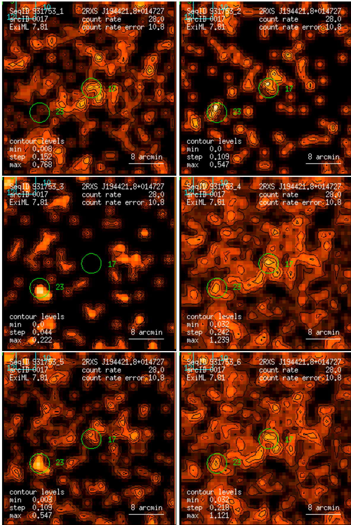
Figure 17: RASS 931753: detection 0017: band rate images, Gaussian filter: (1) PSPC channels 11 – 41, (2) 52 – 90, (3) 91 – 201, (4) 11 – 235, (5) 52 – 201, (6) 11 – 201. Broad band rates in counts/ks. Band rate contour levels in counts/ks/arcmin 2 .
