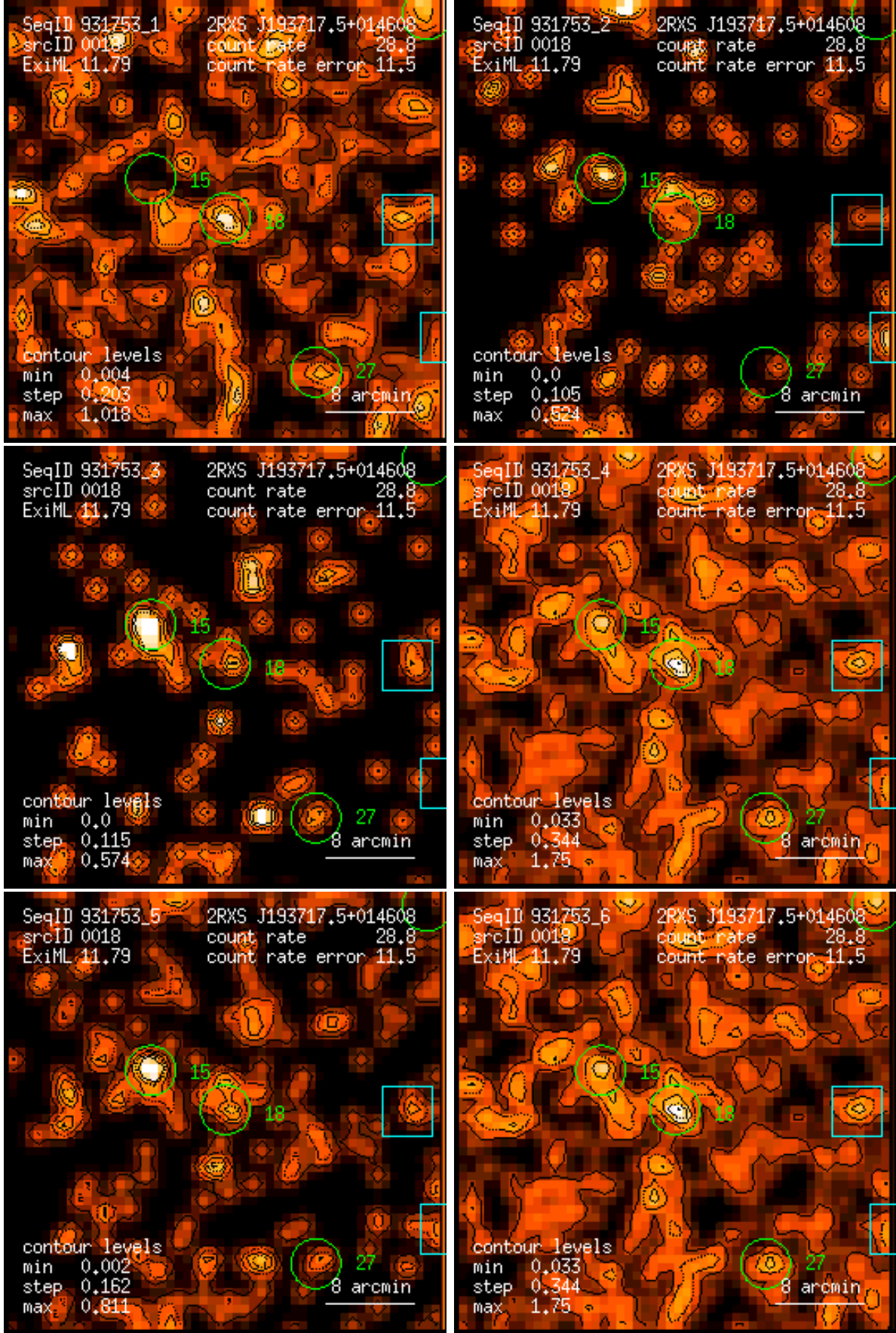
Figure 18: RASS 931753: detection 0018: band rate images, Gaussian filter: (1) PSPC channels 11 – 41, (2) 52 – 90, (3) 91 – 201, (4) 11 – 235, (5) 52 – 201, (6) 11 – 201. Broad band rates in counts/ks. Band rate contour levels in counts/ks/arcmin 2 .
