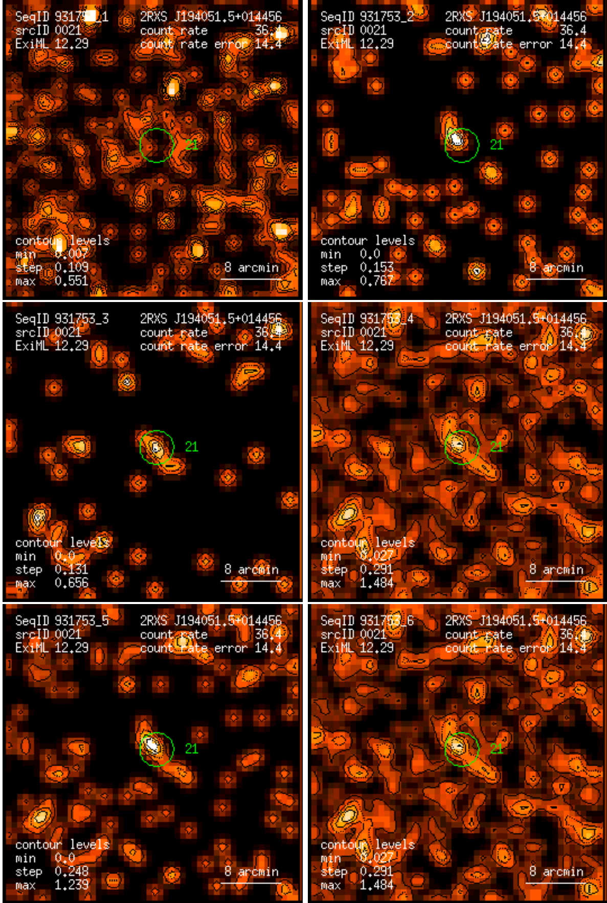
Figure 21: RASS 931753: detection 0021: band rate images, Gaussian filter: (1) PSPC channels 11 – 41, (2) 52 – 90, (3) 91 – 201, (4) 11 – 235, (5) 52 – 201, (6) 11 – 201. Broad band rates in counts/ks. Band rate contour levels in counts/ks/arcmin 2 .
