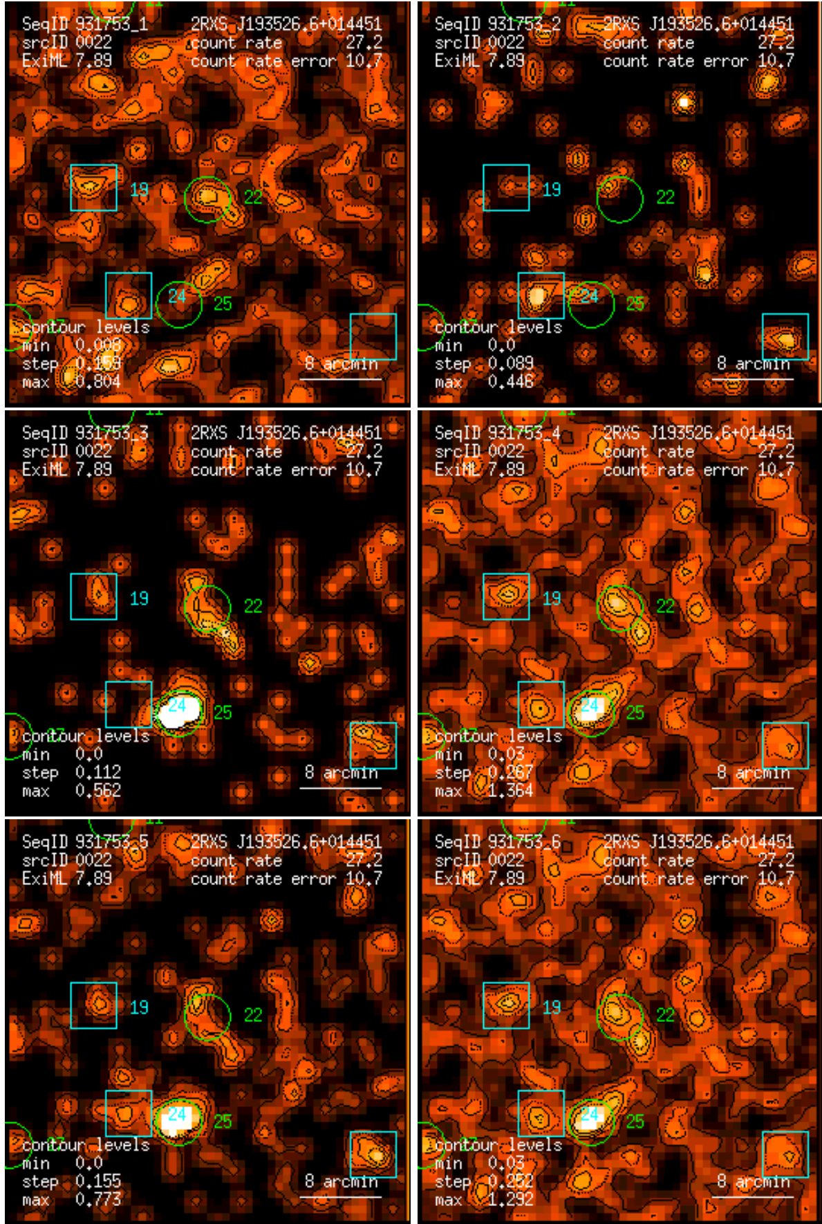
Figure 22: RASS 931753: detection 0022: band rate images, Gaussian filter: (1) PSPC channels 11 – 41, (2) 52 – 90, (3) 91 – 201, (4) 11 – 235, (5) 52 – 201, (6) 11 – 201. Broad band rates in counts/ks. Band rate contour levels in counts/ks/arcmin 2 .
