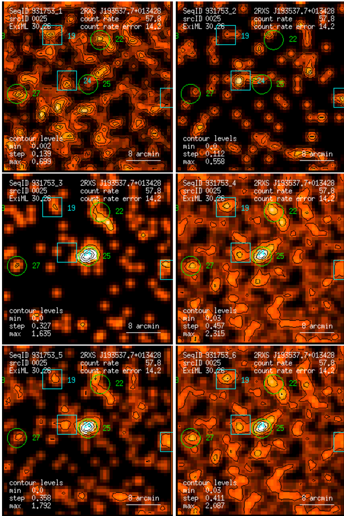
Figure 25: RASS 931753: detection 0025: band rate images, Gaussian filter: (1) PSPC channels 11 – 41, (2) 52 – 90, (3) 91 – 201, (4) 11 – 235, (5) 52 – 201, (6) 11 – 201. Broad band rates in counts/ks. Band rate contour levels in counts/ks/arcmin 2 .
