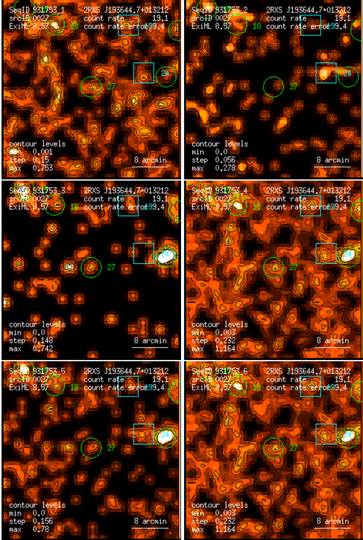
Figure 27: RASS 931753: detection 0027: band rate images, Gaussian filter: (1) PSPC channels 11 – 41, (2) 52 – 90, (3) 91 – 201, (4) 11 – 235, (5) 52 – 201, (6) 11 – 201. Broad band rates in counts/ks. Band rate contour levels in counts/ks/arcmin 2 .
